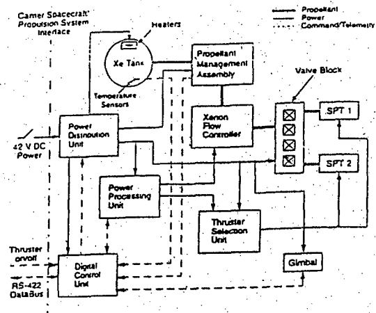
Figure 5: SPT-70 Propulsion System Block Diagram
