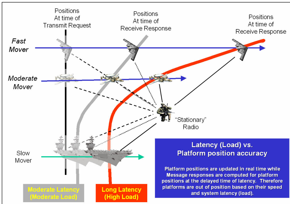
Figure 9 - Platform Position Accuracy
