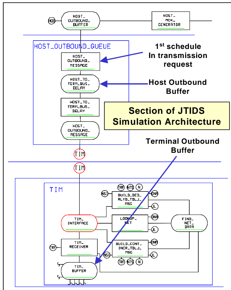
Figure 8 - Section of JTIDS Simulation
