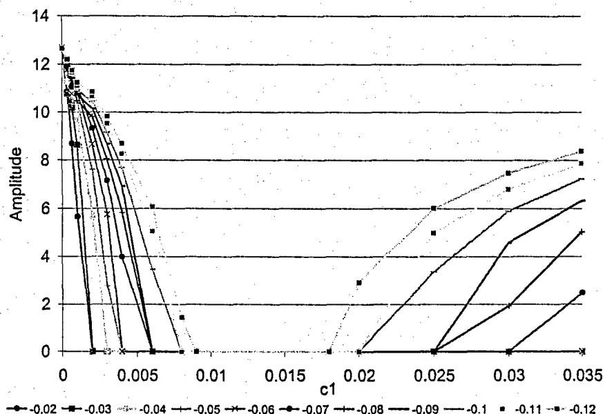
Fig. 2.25 Largest response of mass M_1 as a function of the damping coefficient c_1 for different values of the damping constant c , k_1 = 0.05 , \delta = 0.025 , and \mu = 0 .
