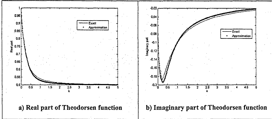
Fig. 2.2 Comparison of the exact Theodorsen function, Eq. (2-12), with its rational approximation, Eq. (2-13)
