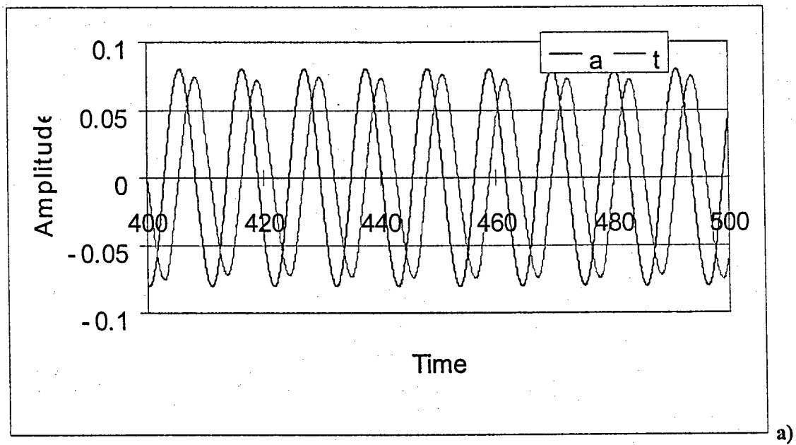
Fig. 3.14: SFSS case, \mu=0.004 , k_d=0.3 Nm/rad
