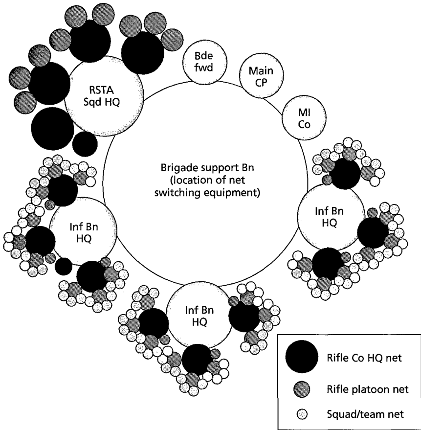
Figure 4.2 Typical Configuration of the SBCT TI
