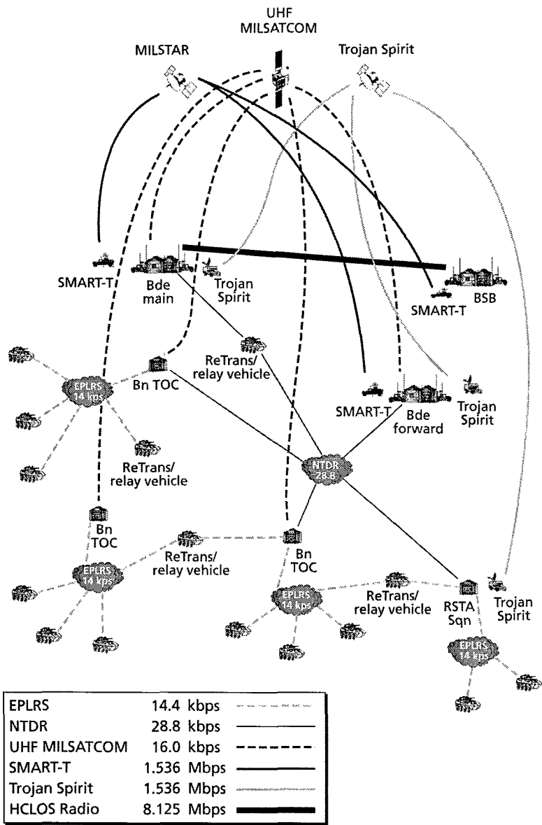
Figure 4.1 Major Elements of the Stryker Brigade Network
