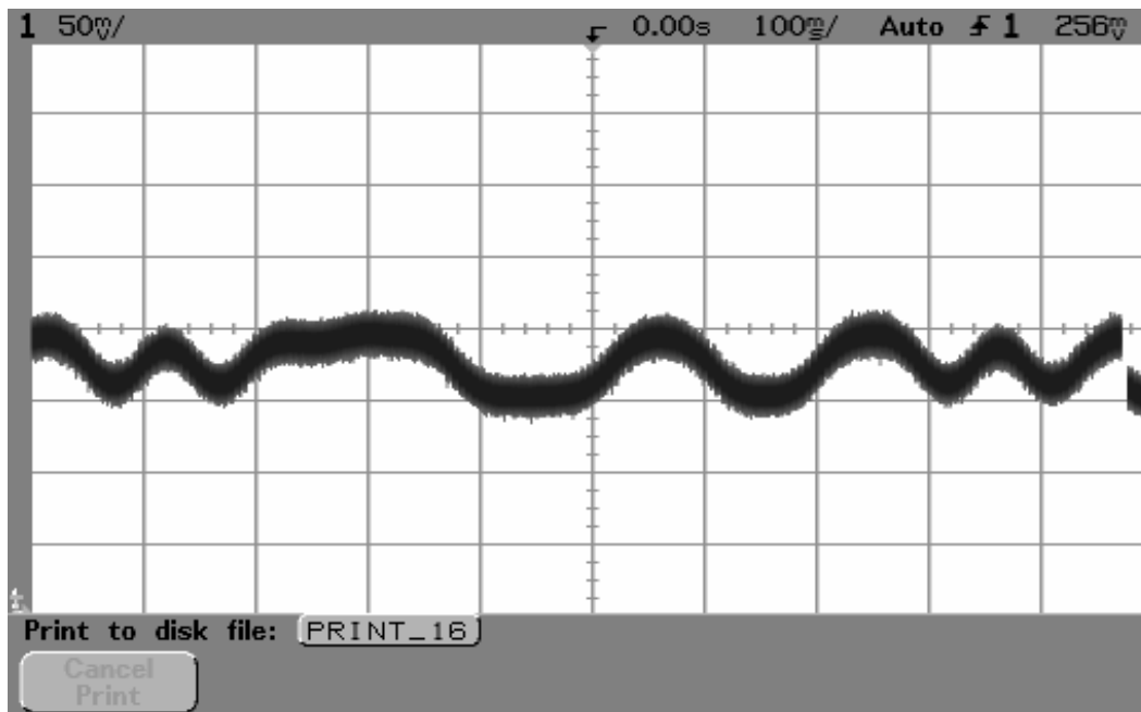
Figure 4.0-17: Watermark PN code with a BER of 7e-3 .
