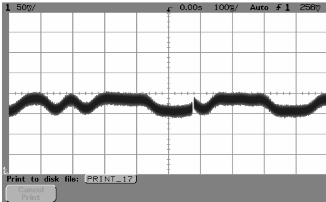
Figure 4.0-18: Watermark PN code with a BER of 8e-2.
