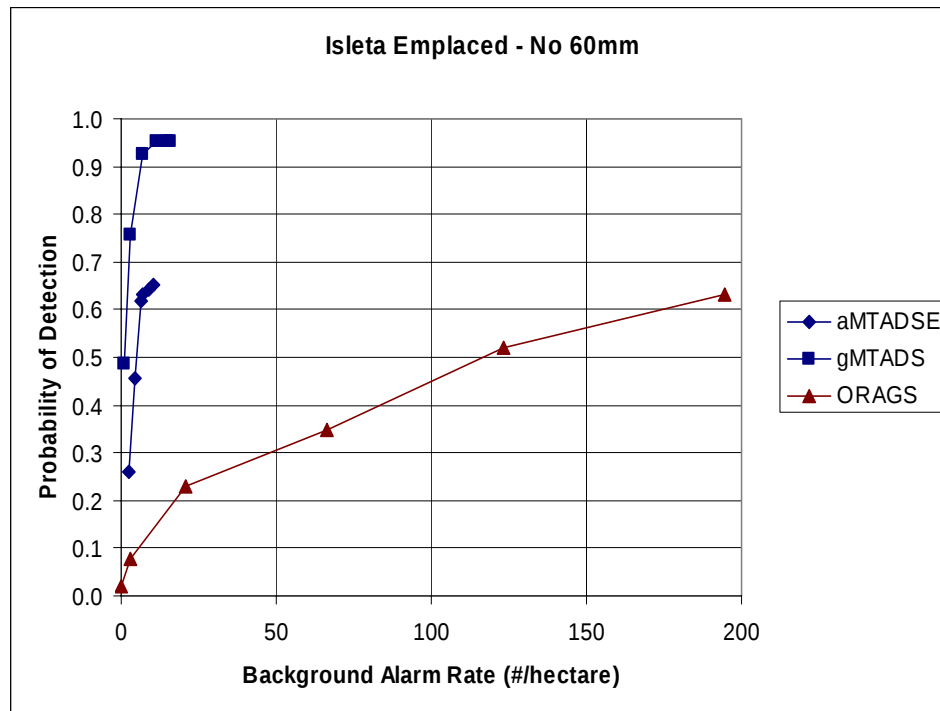
Figure 11. ROC Curves for Isleta Emplaced Ordnance Excluding 60 mm Targets for a 2.0 m Halo
