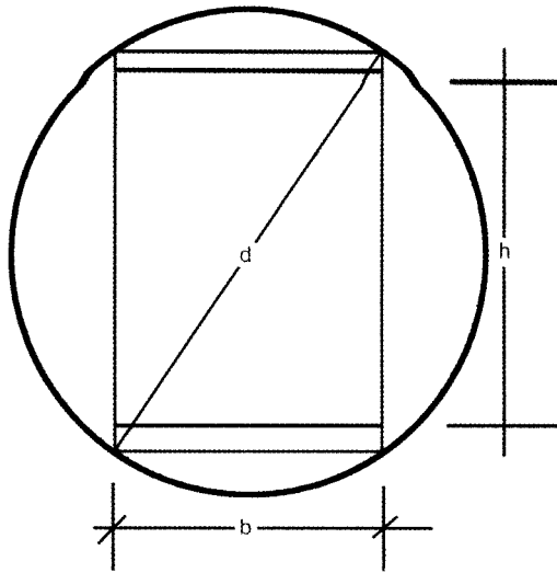
Figure 1. — Rectangular section limited by small-end diameter ( d ) and standard dimensions ( b \times h ).
