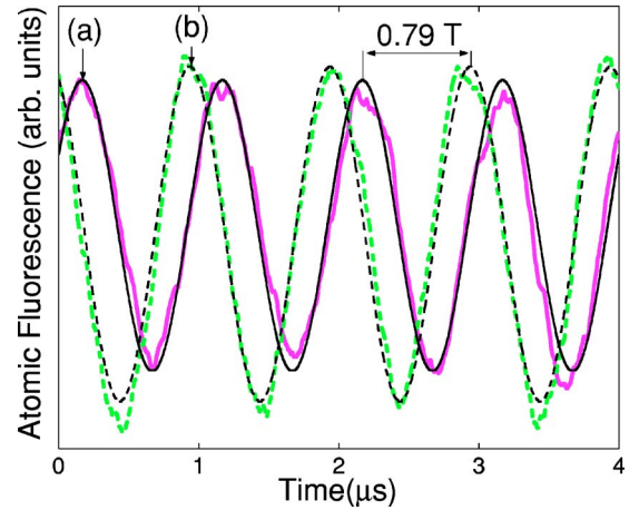
FIG. 5. Demonstration of phase-locked fluorescence. T is the period of the Bloch-Siegert oscillation. (a) Population vs time when a 0.4T delay line was inserted in the reference field cable. (b) Population vs time when the same 0.4T delay line was placed in the fluorescence signal cable. The figure shows that signal (b) is about 0.8T ahead of signal (a), confirming that the atomic fluorescence carries phase information which is locked to the absolute rf field phase. The solid and dashed sinusoidal smooth curves are fittings to the experimental data and were used for period and delay determination.
