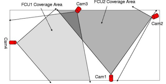
Figure 5: This illustrates the design of two FCUs to cover most of the reachable space within a rectangular room. This enables the system to reliably tracking moving subjects in this room. Two containment units FCU1 and FCU2 are instantiated with two cameras each. The light-shaded and darker-shaded overlays indicate the valid triangulation regions for FCU1 and FCU2 respectively. The two FCU regions overlap each other (highlighted with the darkest shade). In general, the cameras do not have fixed orientation, and other FCU instantiations are possible.
