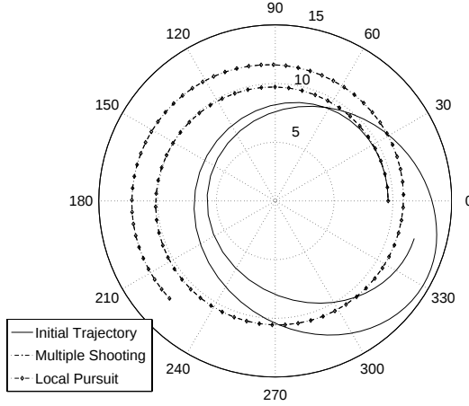
Fig. 4. Trajectories of both methods under well-conditioned case with N = 101, N_{\Delta} = 30, N_{\delta} = 16 . The trajectories obtained from both methods were virtually identical.
