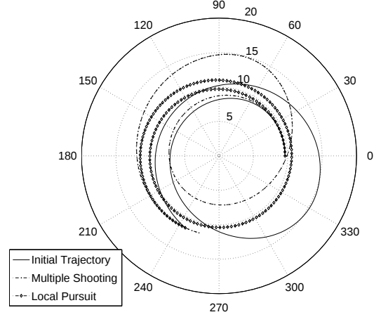
Fig. 5. Trajectories under ill-conditioned case with selection of N = 201, N_{\Delta} = 30, N_{\delta} = 16 . The trajectory obtained from local pursuit was essentially optimal, while the one obtained from multiple shooting was far away from optimum.
