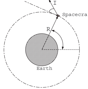
Fig. 3. A planar spacecraft in orbit around the Earth.
