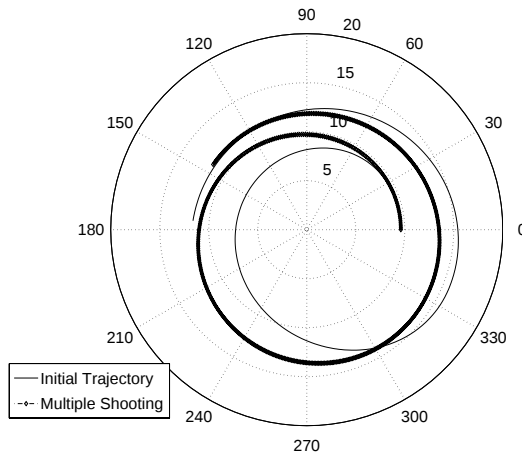
Fig. 6. Spacecraft trajectory in the case of large number of segments, N = 601 , N_{\Delta} = 60 , N_{\delta} = 32 .
