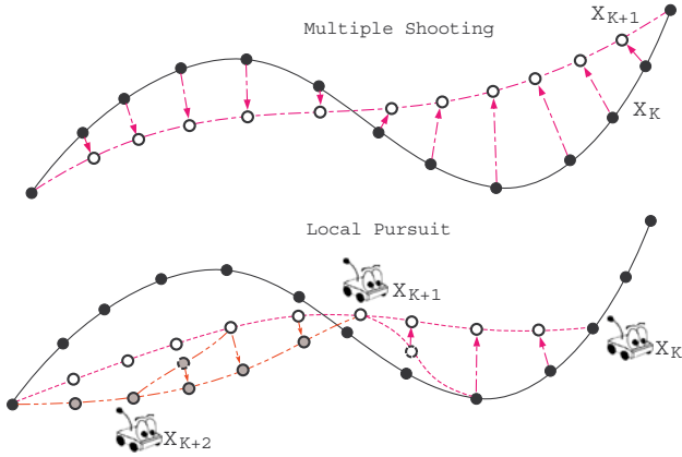
Fig. 2. Local pursuit could decrease the problem size involved in calculation at every updating step. The number of variables calculated in multiple shooting is N = 13 , and the number of variables calculated by each agent in local pursuit is N_\Delta = 5 .
