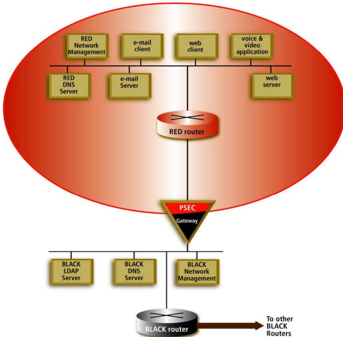
Figure 4. Coalition LAN
