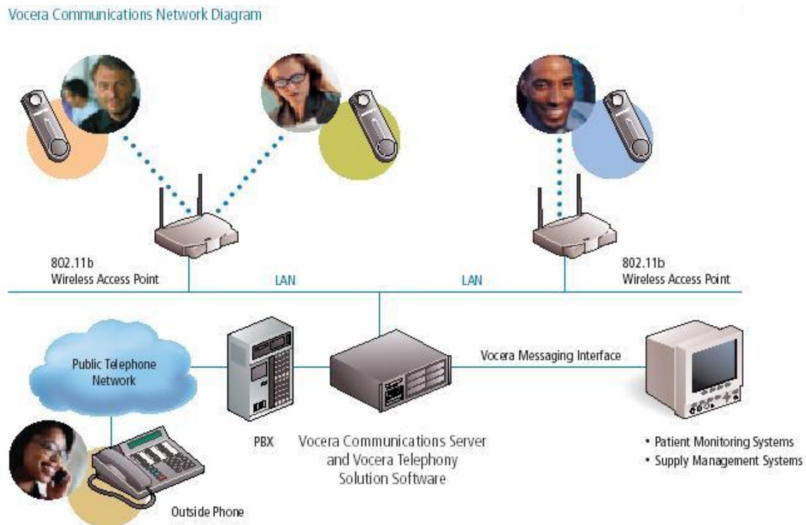
Figure 55. Vocera sample topology (From Ref. 91 )
