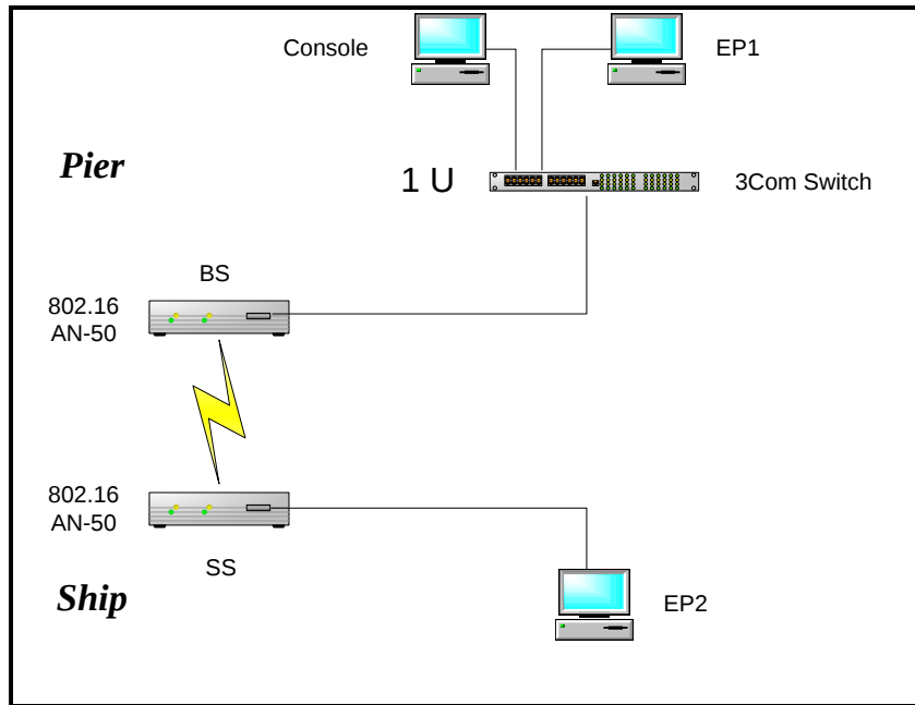
Figure 8. Pier-to-Ship Control Network Diagram
