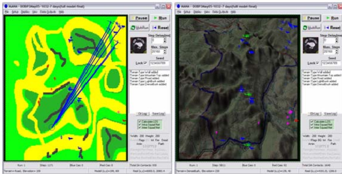
Figure 16. This shows two different views of the simulation running. On the left is artillery firing with the terrain map displayed. On the right is a resupply with the scenario background. [Best viewed in color]
