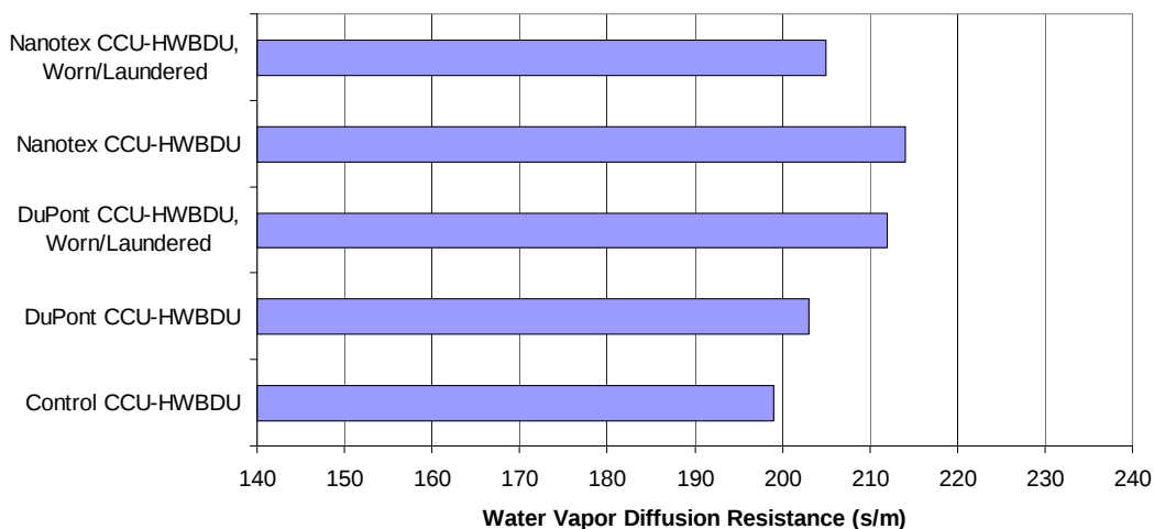
Figure 15. Water vapor diffusion resistance. Slight differences between the Control and the DuPont or Nanotex water-repellent treatments.
