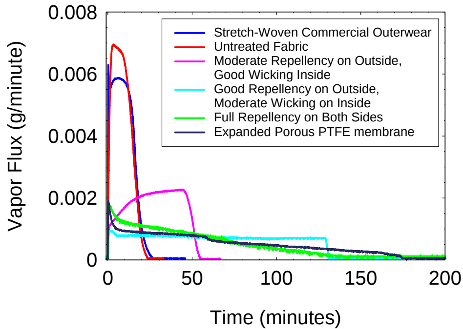
Figure 23. Drying curves for differential DWR fabric treatments.
