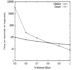
Fig. 11. Runtime ( sports ).
