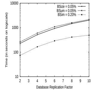
Fig. 19. scalability ( T30I15D100Kx ).
