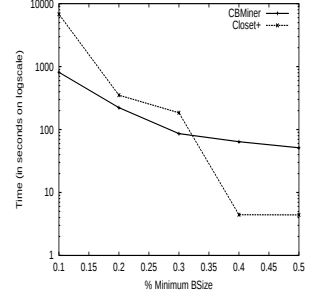
Fig. 9. Runtime ( T40I10D100K ).
