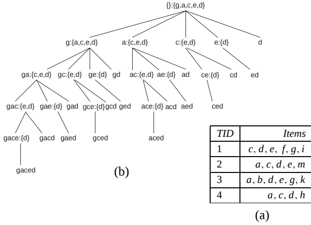
Figure 1: (a) A transaction database with \theta \geq 0.5 ; (b) The pattern tree.
