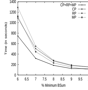
Fig. 16. Pruning methods. ( pumsb* ).
