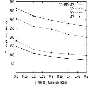
Fig. 17. Pruning methods. ( big-market ).
