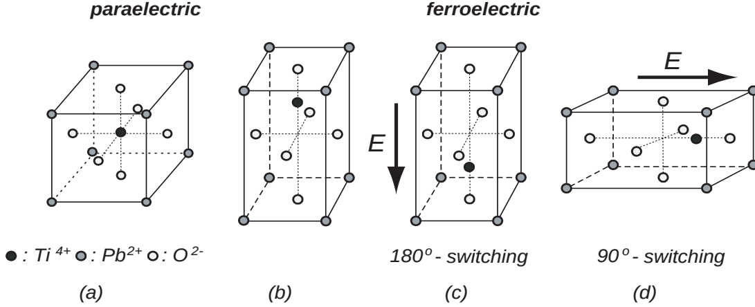
Fig. 1. Lattice structure in a paraelectric and ferroelectric PbTiO_3 crystal, 90°- and 180°-switching processes.
