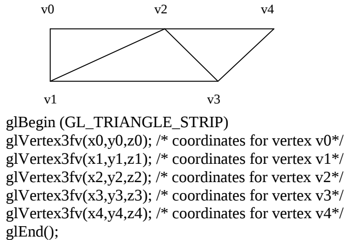
Figure 2: Example of using GL_TRIANGLE_STRIP primitive.
