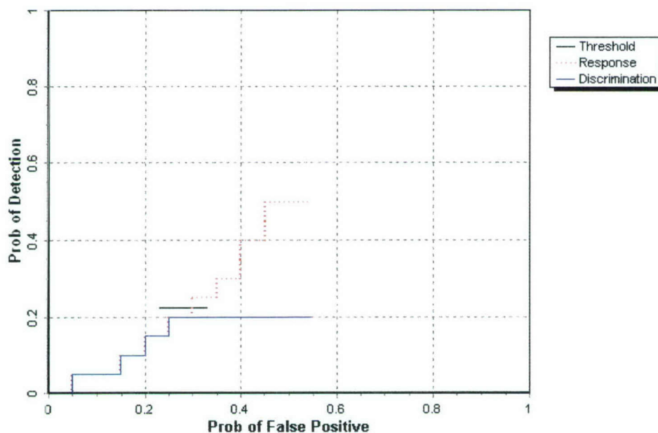
Figure 2. EM61 MKII/man-portable wooded area probability of detection for response and discrimination stages versus their respective probability of false positive over all ordnance categories combined.
