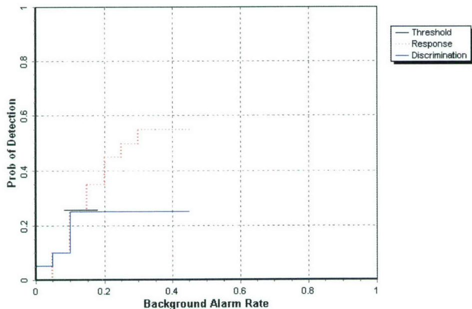
Figure 5. EM61 MKII/Man-Portable wooded area probability of detection for response and discrimination stages versus their respective background alarm rate for all ordnance larger than 20 mm.
