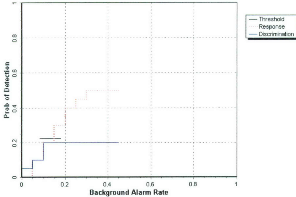
Figure 3. EM61 MKII/Man-Portable wooded area probability of detection for response and discrimination stages versus their respective background alarm rate over all ordnance categories combined.
