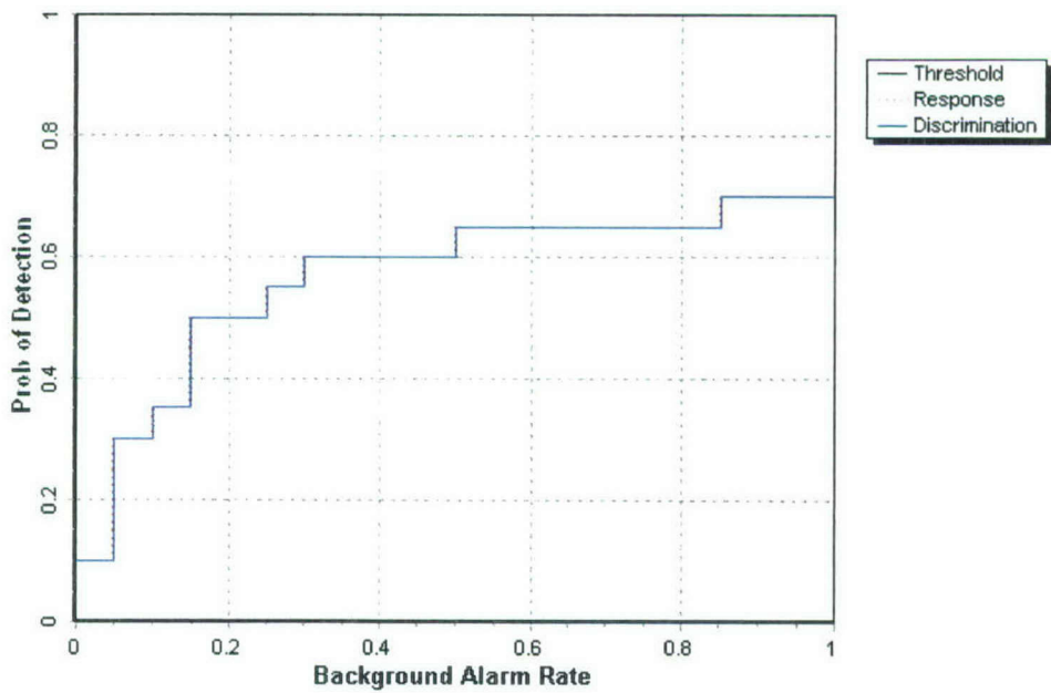
Figure 11. Simultaneous Magnetometry open field probability of detection for response and discrimination stages versus their respective background alarm rate for all ordnance larger than 20 mm.
