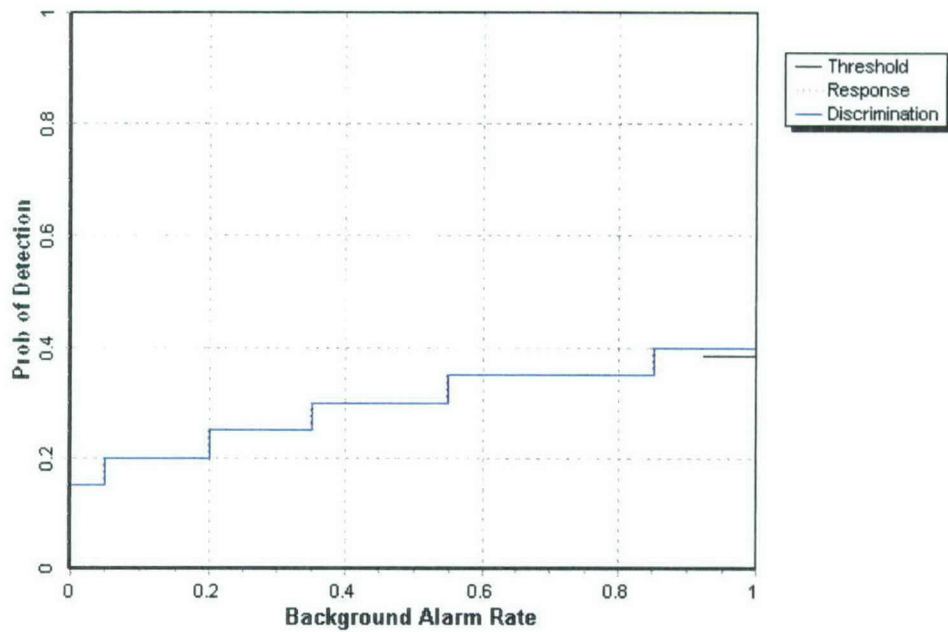
Figure 3. Pulsed EM open field probability of detection for response and discrimination stages versus their respective background alarm rate over all ordnance categories combined.
