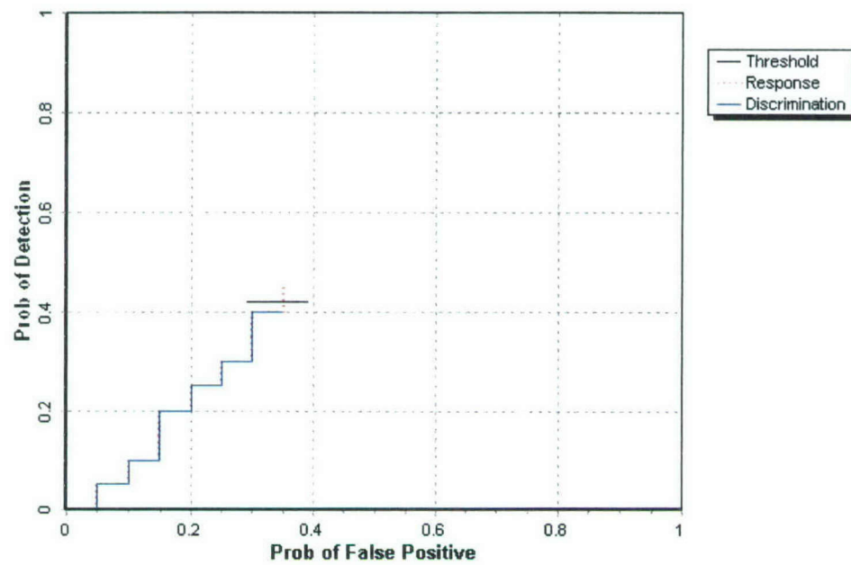
Figure 8. Pulsed EM open field probability of detection for response and discrimination stages versus their respective probability of false positive for all ordnance larger than 20 mm.
