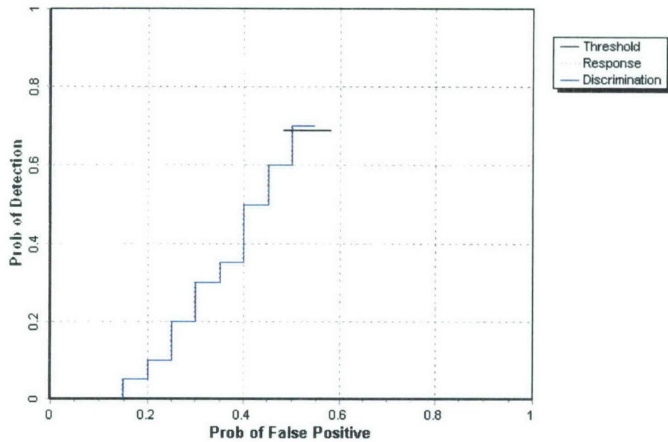
Figure 10. Simultaneous Magnetometry open field probability of detection for response and discrimination stages versus their respective probability of false positive for all ordnance larger than 20 mm.
