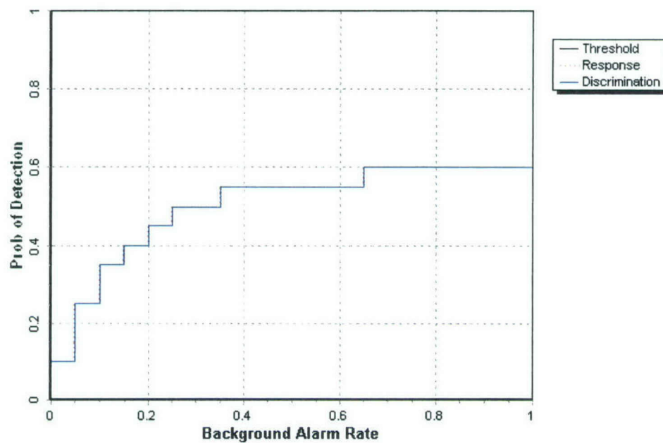
Figure 5. Simultaneous Magnetometry open field probability of detection for response and discrimination stages versus their respective background alarm rate over all ordnance categories combined.
