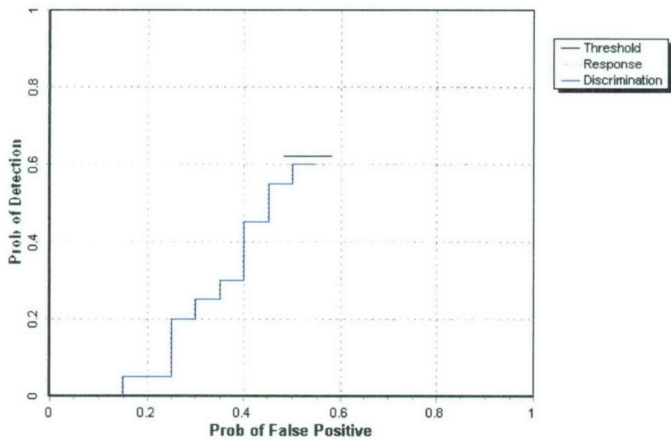
Figure 4. Simultaneous Magnetometry open field probability of detection for response and discrimination stages versus their respective probability of false positive over all ordnance categories combined.
