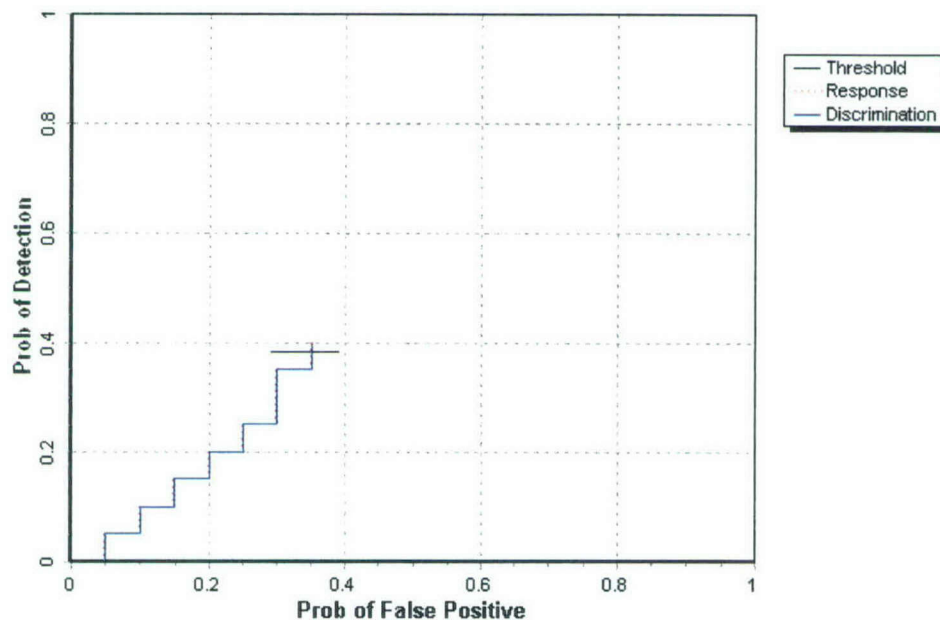
Figure 2. Pulsed EM open field probability of detection for response and discrimination stages versus their respective probability of false positive over all ordnance categories combined.
