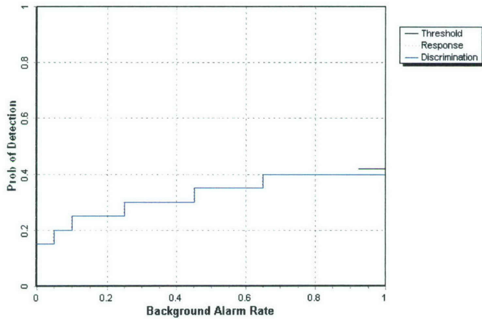
Figure 9. Pulsed EM open field probability of detection for response and discrimination stages versus their respective background alarm rate for all ordnance larger than 20 mm.
