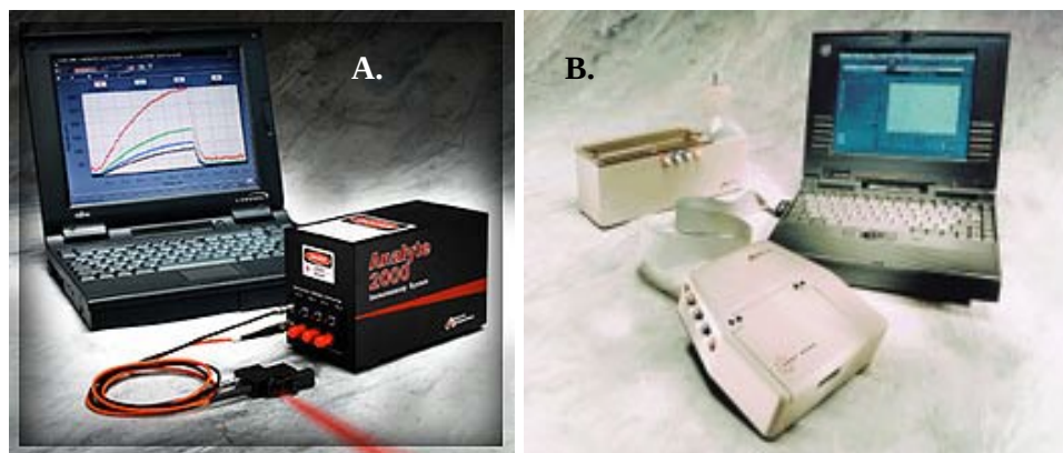
Figure 10. (A) The Fast 2000 TM and (B) Analyte 2000 TM immunosensors. Photos used with permission.
