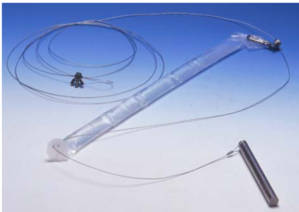
Figure 1. The passive diffusion bag sampler. Photo used with permission. ( http://www.caslab.com/products.php )
