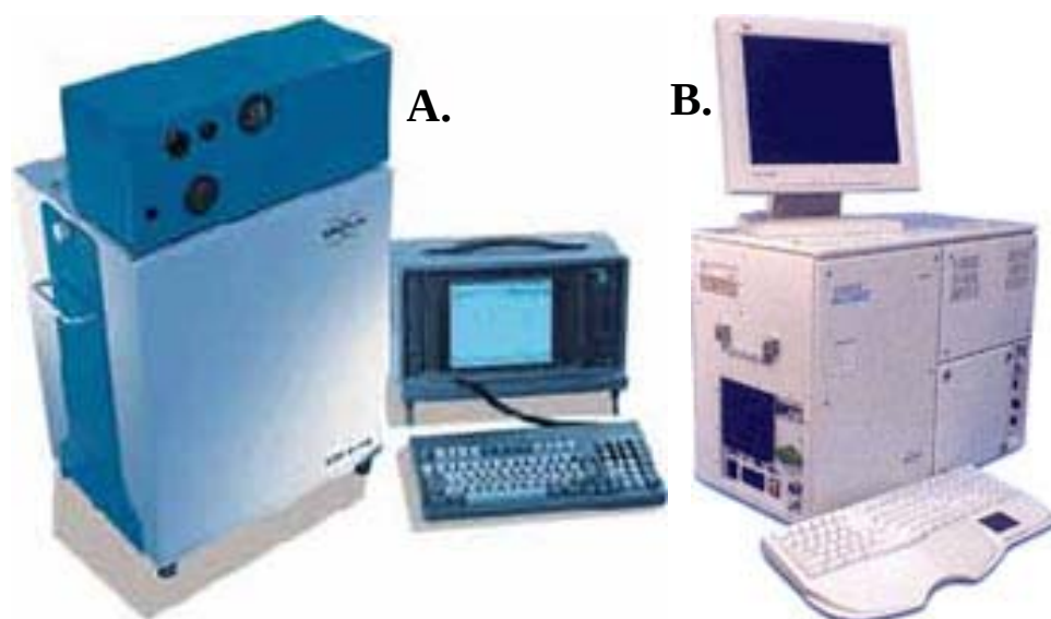
Figure 6. Transportable GC/MS instruments (A) EM640™ Mobile GC/MS; (B) The Viking 573 GC/MS. ( http://www.bdal.de/modux3/ ). Photos used with permission.
