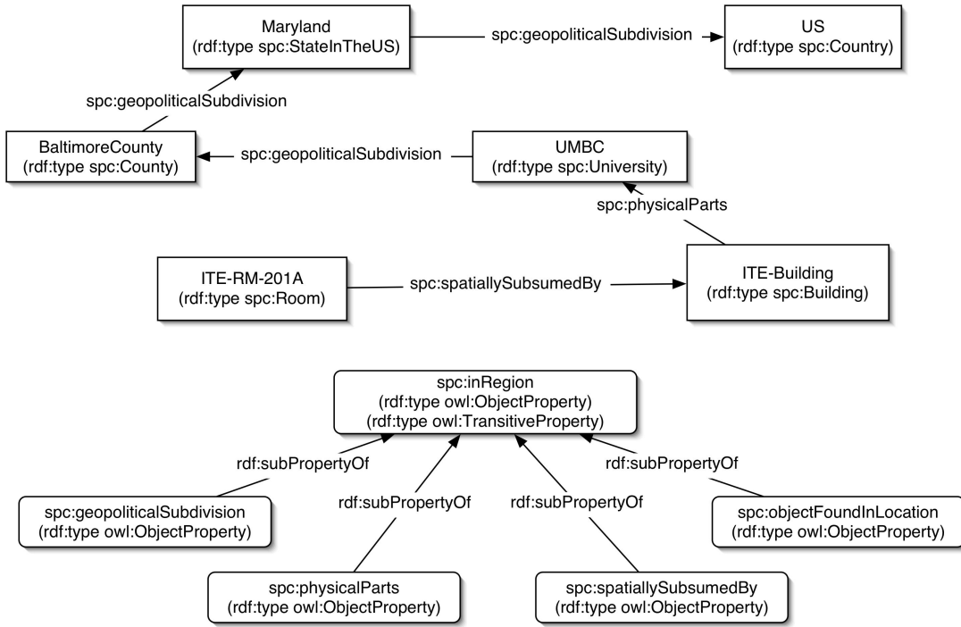
Figure 4: A simple spatial ontology about UMBC is defined using COBRA-ONT. This ontology enables the Context Broker to reason about the location context of a device or a person. Ontologies are shared between the Context Broker and other computing entities in the space.
