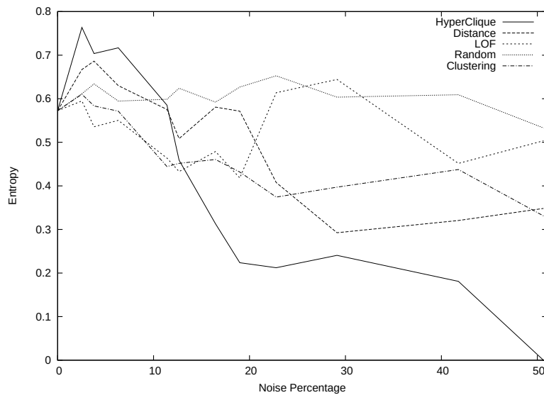
Fig. 6. The impact of noise removal techniques on the performance of clustering analysis for the yeast gene expression data in terms of entropy.
