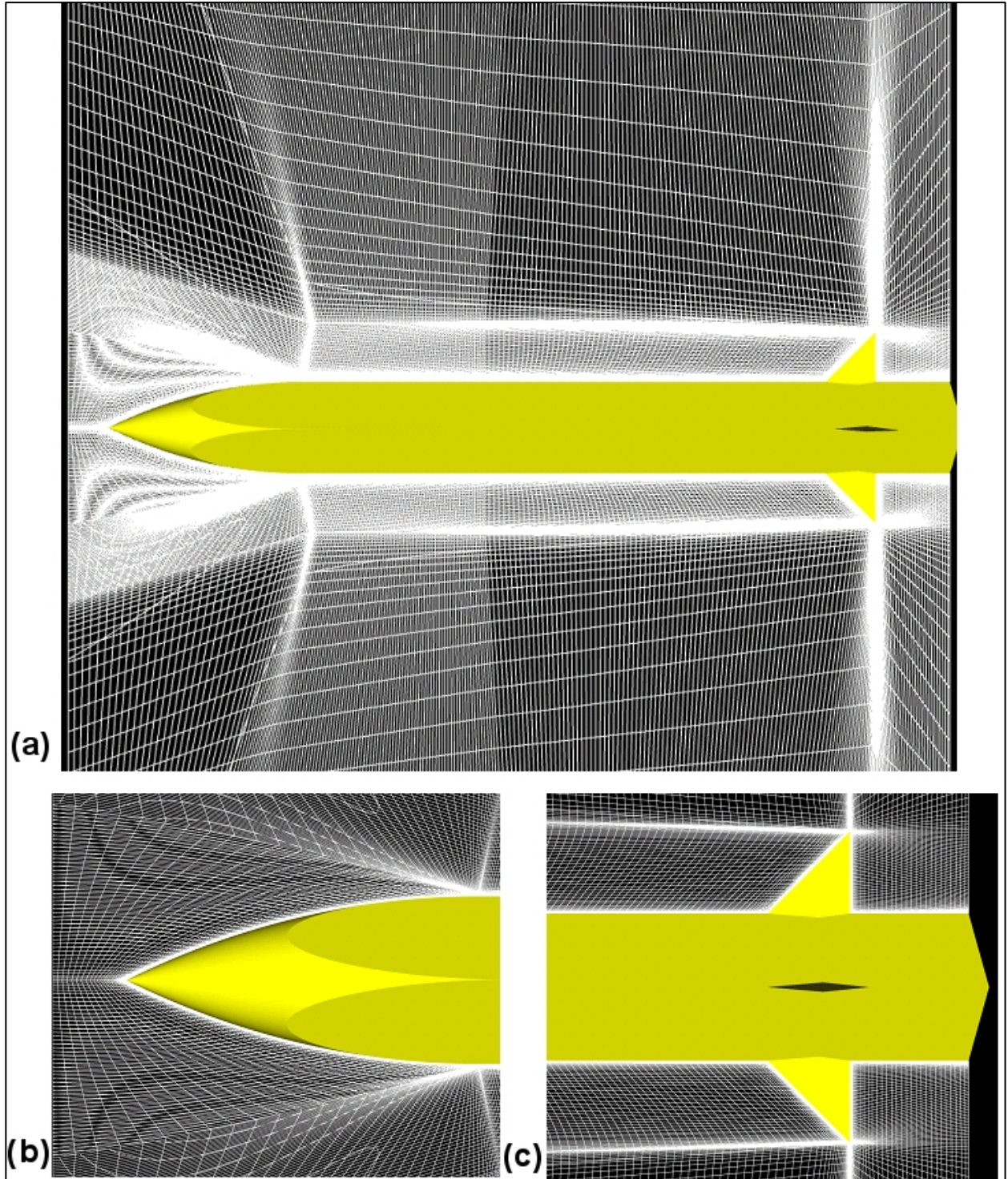
Figure 5. (a) Computational grid for corner fin geometry with y^+ = 30 spacing. Close-up of (b) nose tip and (c) fins.
