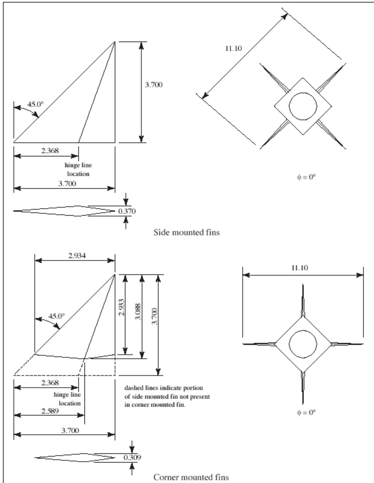
Figure 2. Sketch (inches) of side and corner mounted tail fins (17).
