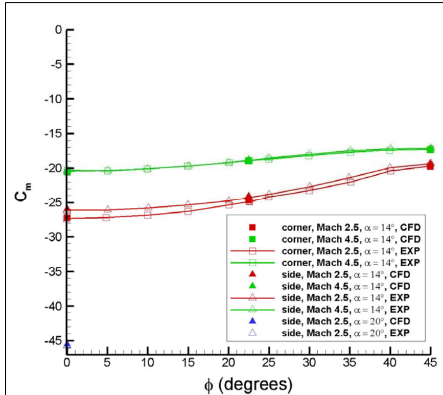
Figure 13. Pitching moment coefficient as a function of roll orientation.
