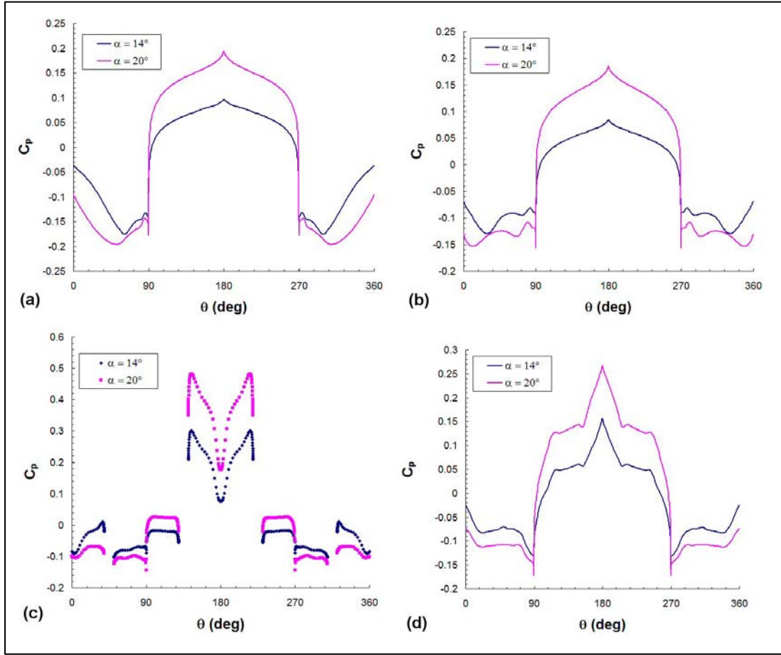
Figure 24. Pressure coefficient distribution for Mach 2.5 and \phi = 0^\circ at (a) x/D = 5.5 , (b) x/D = 8.5 , (c) x/D = 11.5 , and (d) x/D = 12.5 .
