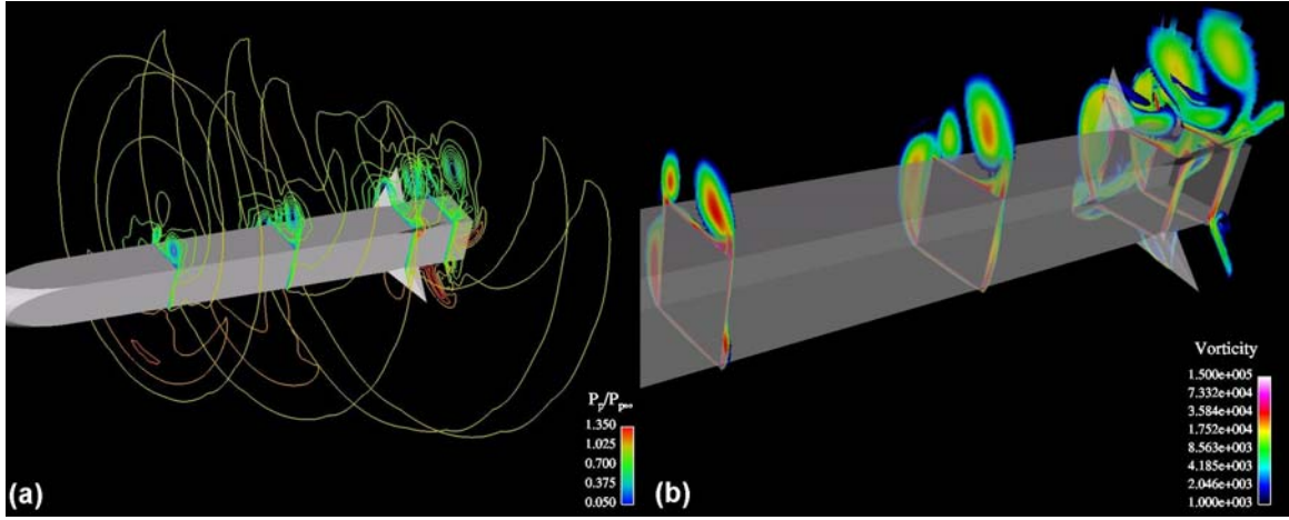
Figure 27. Three-dimensional (a) pitot pressure contours and (b) vorticity contours for corner fin configuration, Mach 2.5, \phi = 22.5^\circ , \alpha = 14^\circ .
