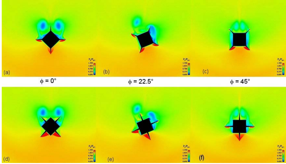
Figure 42. Pressure contours for ([a]–[c]) corner fin configuration and ([d]–[f]) side fin configuration at roll orientations indicated Mach 2.5, \alpha = 14^\circ , x/D = 11.5 .
