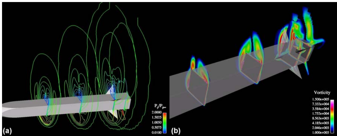
Figure 34. Three-dimensional (a) pitot pressure contours and (b) vorticity contours for corner fin configuration, Mach 4.5, \phi = 22.5^\circ , \alpha = 14^\circ .
