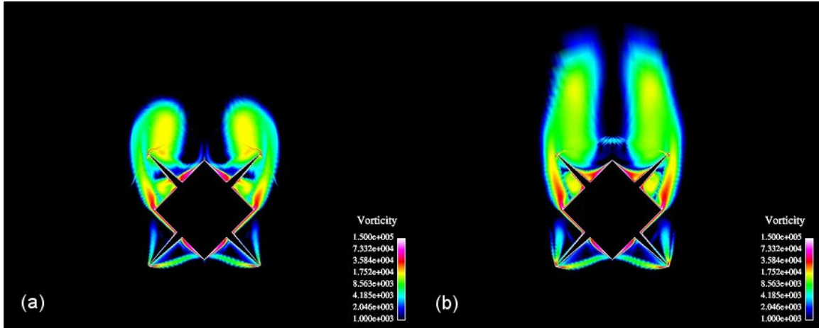
Figure 47. Vorticity contours for side fin configuration at Mach 2.5, \phi = 0^\circ , x/D = 11.5 , (a) \alpha = 14^\circ and (b) \alpha = 20^\circ .
