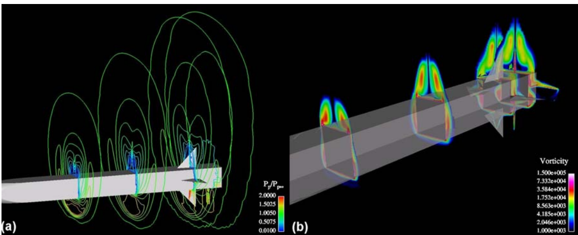
Figure 37. Three-dimensional (a) pitot pressure contours and (b) vorticity contours for side fin configuration, Mach 4.5, \phi = 45^\circ , \alpha = 14^\circ .
