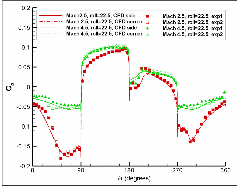
Figure 17. Pressure coefficient distribution at x/D = 5.5 , \phi = 22.5^\circ , \alpha = 14^\circ .
