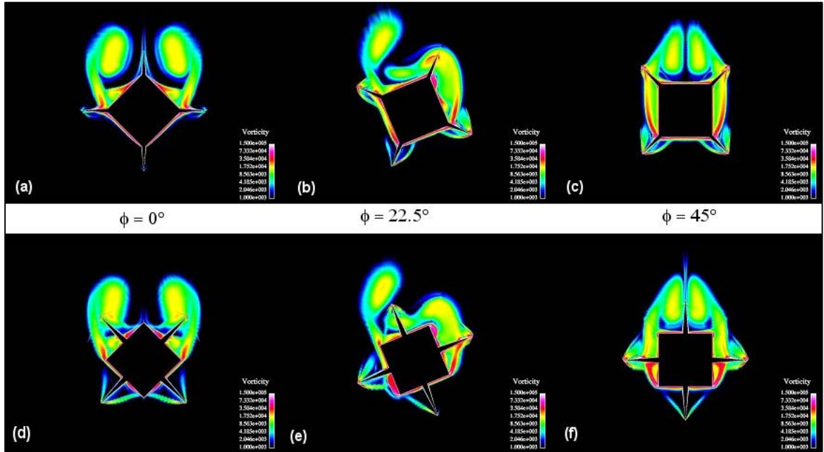
Figure 43. Vorticity contours for ([a] – [c]) corner fin configuration and ([d] – [f]) side fin configuration at roll orientations indicated for Mach 2.5, \alpha = 14^\circ , x/D = 11.5 .
