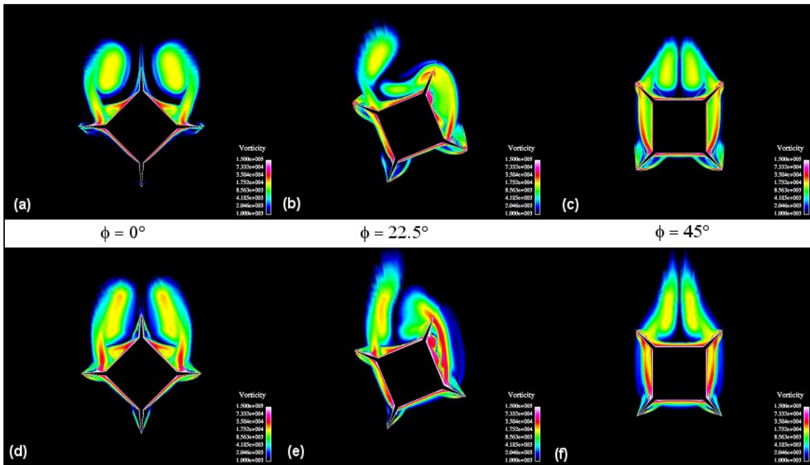
Figure 44. Vorticity contours for corner fin configuration at roll orientations indicated, \alpha = 14^\circ , x/D = 11.5 for ([a]–[c]) Mach 2.5 and ([d]–[f]) Mach 4.5.
