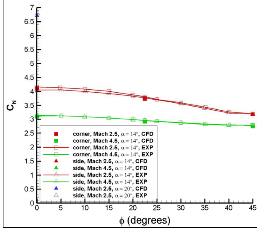
Figure 10. Normal force coefficient as a function of roll orientation.
