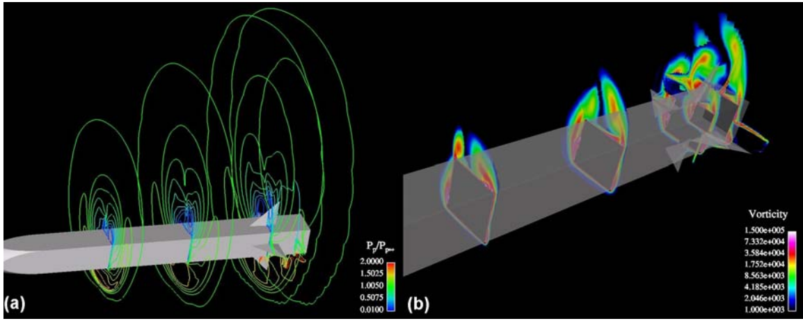
Figure 35. Three-dimensional (a) pitot pressure contours and (b) vorticity contours for side fin configuration, Mach 4.5, \phi = 22.5^\circ , \alpha = 14^\circ .
