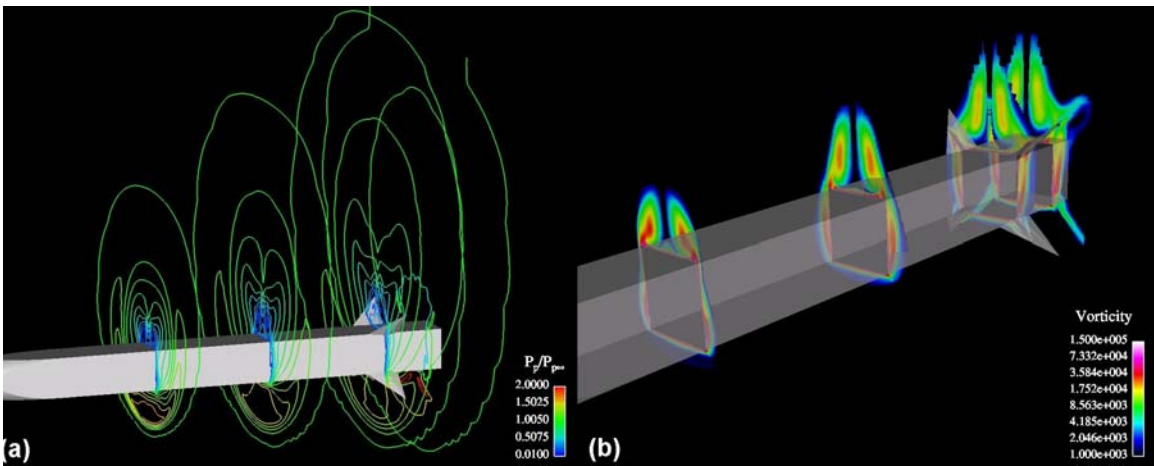
Figure 36. Three-dimensional (a) pitot pressure contours and (b) vorticity contours for corner fin configuration, Mach 4.5, \phi = 45^\circ , \alpha = 14^\circ .
