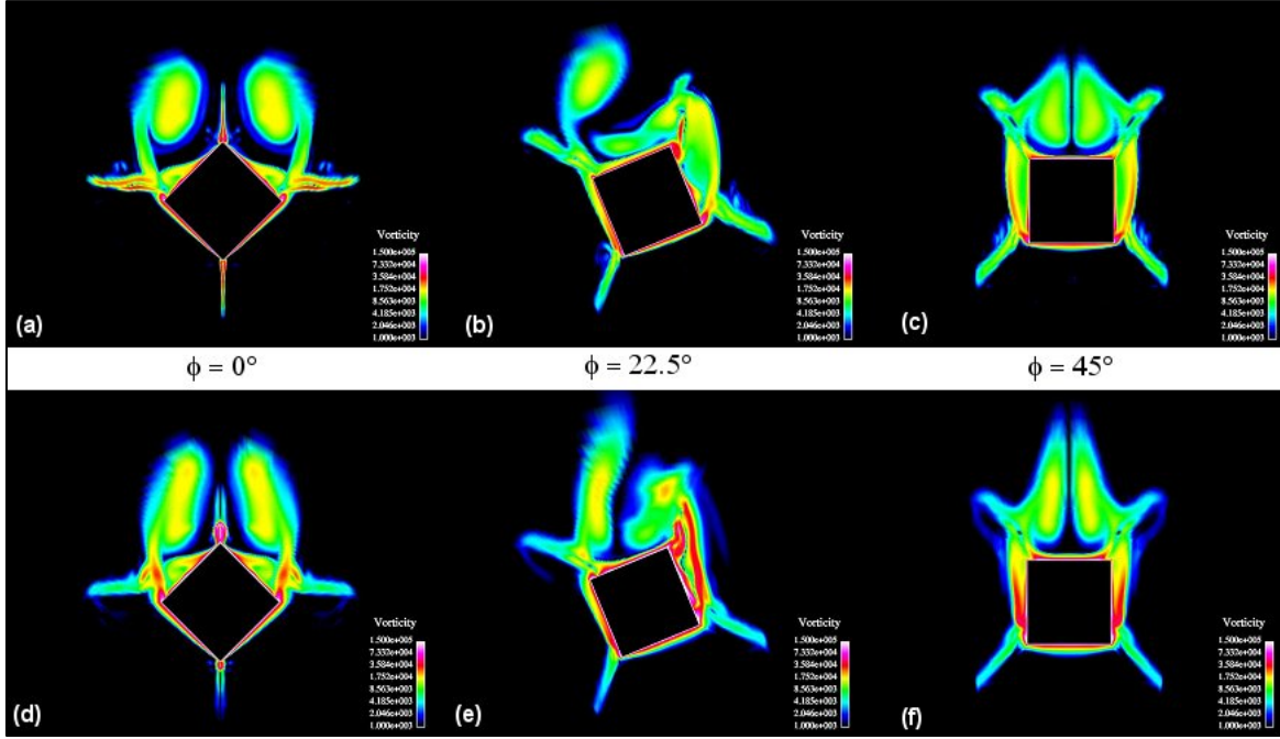
Figure 45. Vorticity contours for corner fin configuration at roll orientations indicated, \alpha = 14^\circ , x/D = 12.5 for ([a]–[c]) Mach 2.5 and ([d]–[f]) Mach 4.5.
