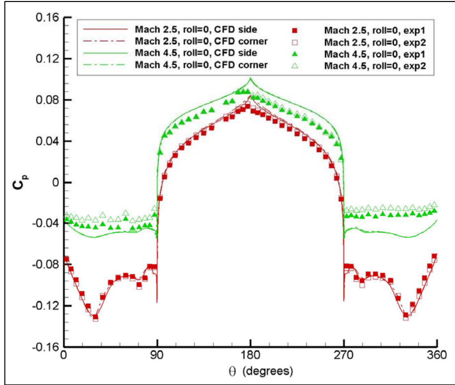
Figure 19. Pressure coefficient distribution at x/D = 8.5 , \phi = 0^\circ , \alpha = 14^\circ .
