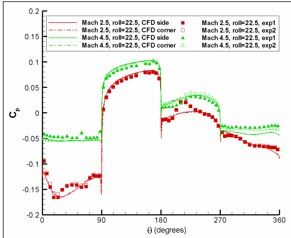
Figure 20. Pressure coefficient distribution at x/D = 8.5 , \phi = 22.5^\circ , \alpha = 14^\circ .
