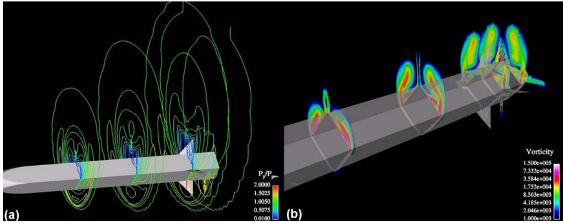
Figure 32. Three-dimensional (a) pitot pressure contours and (b) vorticity contours for corner fin configuration, Mach 4.5, \phi = 0^\circ , \alpha = 14^\circ .
