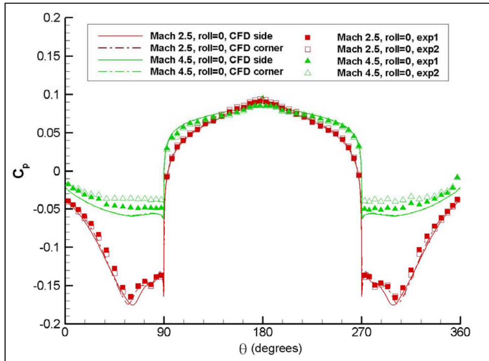
Figure 16. Pressure coefficient distribution at x/D = 5.5 , \phi = 0^\circ , \alpha = 14^\circ .
