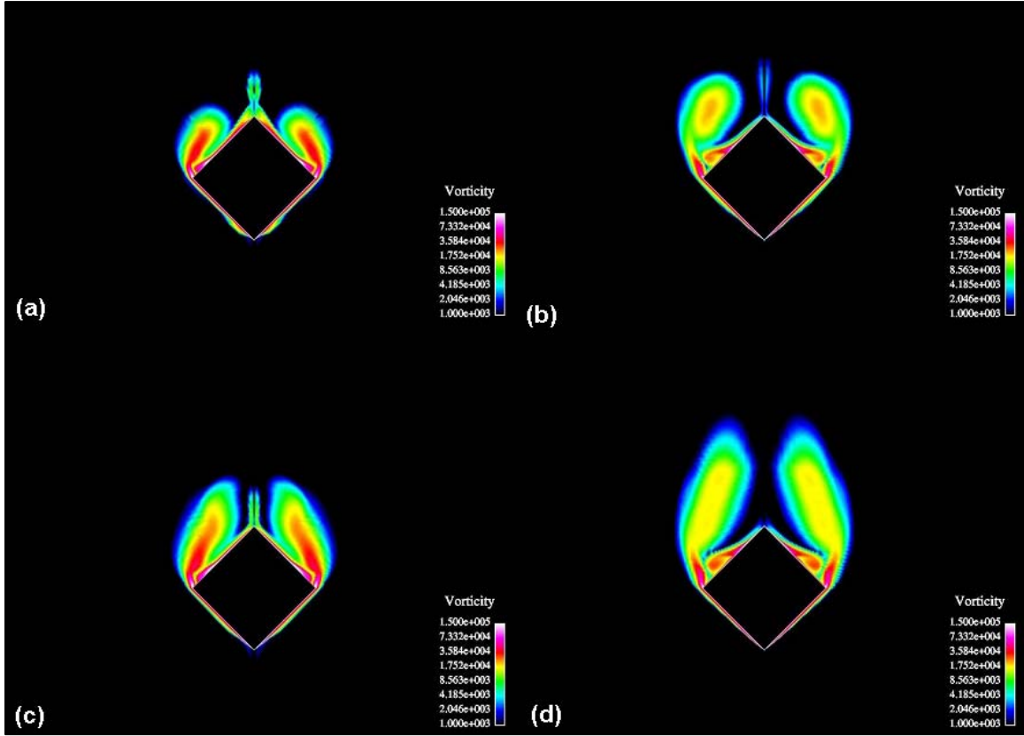
Figure 40. Vorticity contour plots for side fin configuration at Mach 2.5, \phi = 0^\circ , ([a]–[b]) \alpha = 14^\circ , x/D = 5.5 and 8.5 , respectively, and ([c]–[d]) \alpha = 20^\circ , x/D = 5.5 and 8.5 , respectively.
