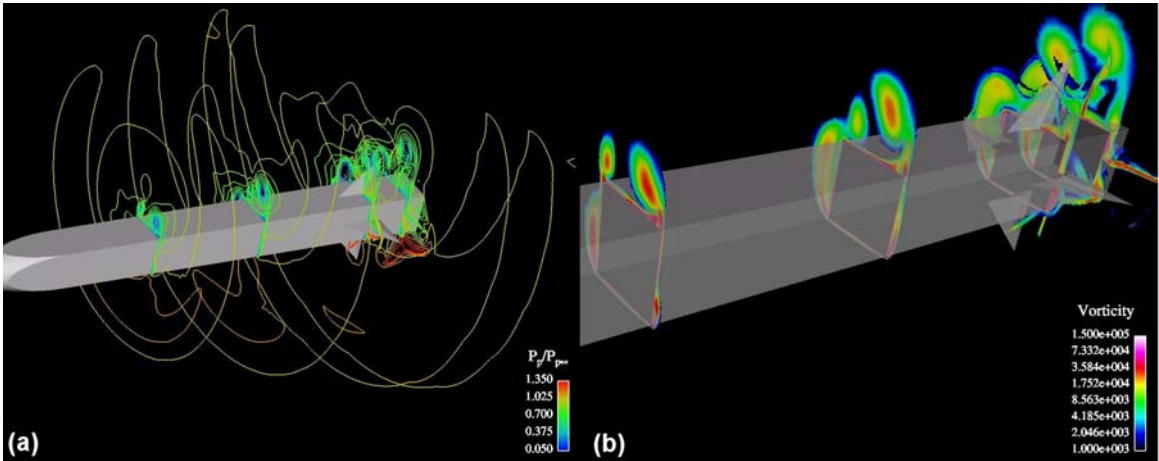
Figure 28. Three-dimensional (a) pitot pressure contours and (b) vorticity contours for side fin configuration, Mach 2.5, \phi = 22.5^\circ , \alpha = 14^\circ .
