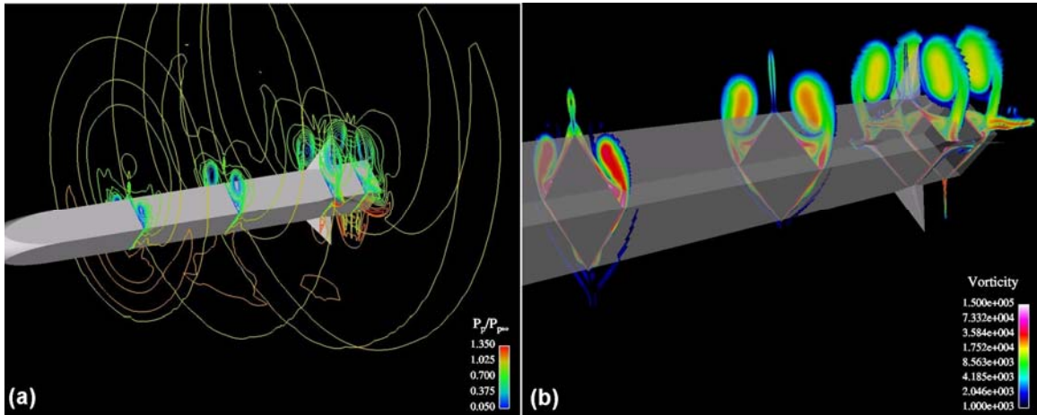
Figure 25. Three-dimensional (a) pitot pressure contours and (b) vorticity contours for corner fin configuration, Mach 2.5, \phi = 0^\circ , \alpha = 14^\circ .
