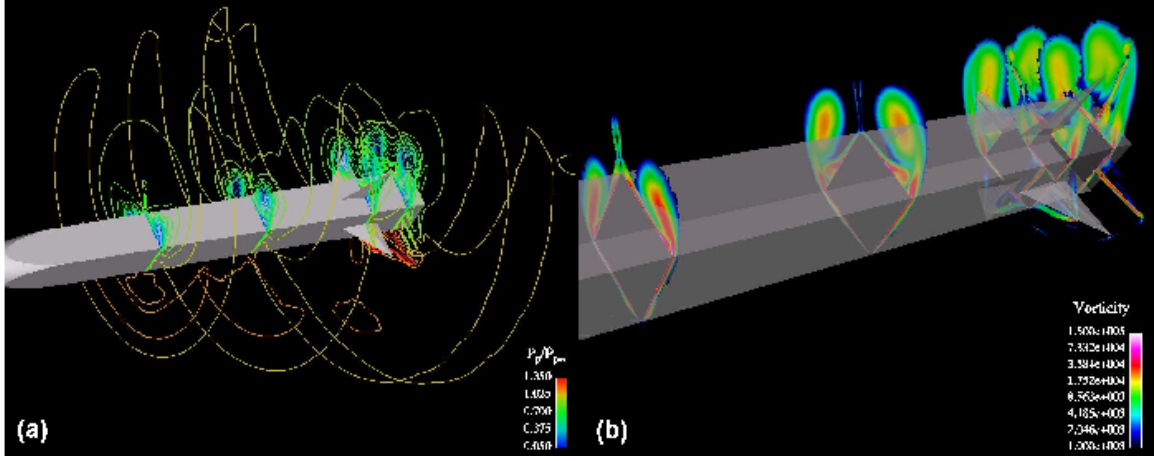
Figure 26. Three-dimensional (a) pitot pressure contours and (b) vorticity contours for side fin configuration, Mach 2.5, \phi = 0^\circ , \alpha = 14^\circ .
