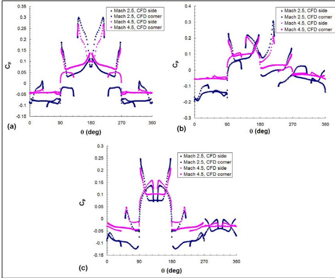
Figure 22. Pressure coefficient distribution at x/D = 11.5 . (a) \phi = 0^\circ , \alpha = 14^\circ , (b) \phi = 22.5^\circ , \alpha = 4^\circ , (c) \phi = 45^\circ , \alpha = 14^\circ .
