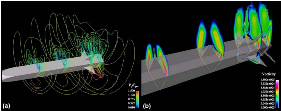
Figure 31. Three-dimensional (a) pitot pressure contours and (b) vorticity contours for side fin configuration, Mach 2.5, \phi = 0^\circ , \alpha = 20^\circ .
