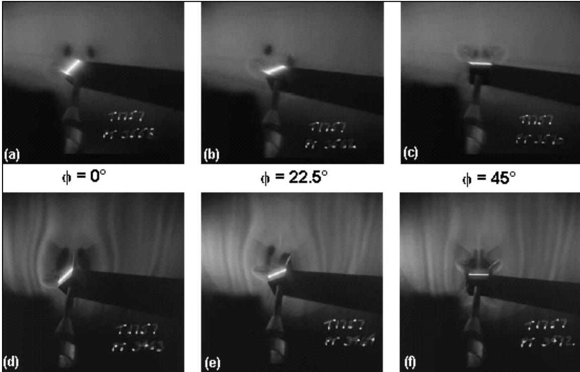
Figure 46. Experimental vapor screen images for corner fin configuration at roll orientations indicated, \alpha = 14^\circ , x/D = 12.5 for ([a]–[c]) Mach 2.5 and ([d]–[f]) Mach 4.5.
