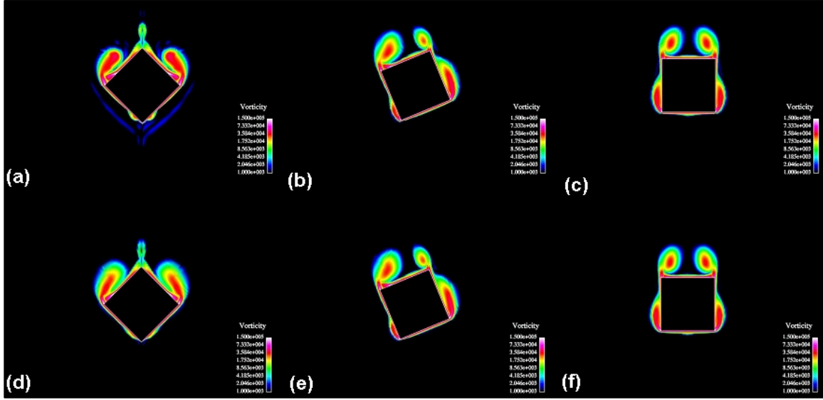
Figure 38. Vorticity contour plots at x/D = 5.5 , Mach 2.5, \alpha = 14^\circ for ([a]–[c]) corner fin configuration \phi = 0^\circ, 22.5^\circ, 45^\circ , respectively, and ([d]–[f]) side fin configuration, \phi = 0^\circ, 22.5^\circ, 45^\circ , respectively.
