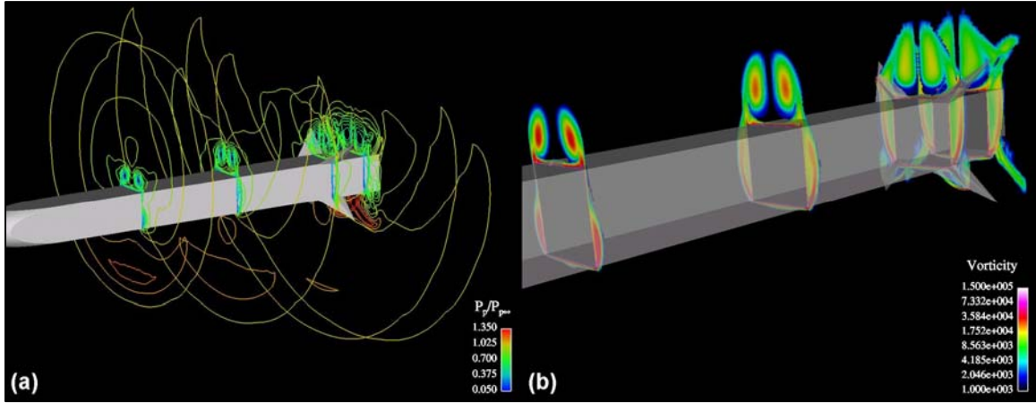
Figure 29. Three-dimensional (a) pitot pressure contours and (b) vorticity contours for corner fin configuration, Mach 2.5, \phi = 45^\circ , \alpha = 14^\circ .
