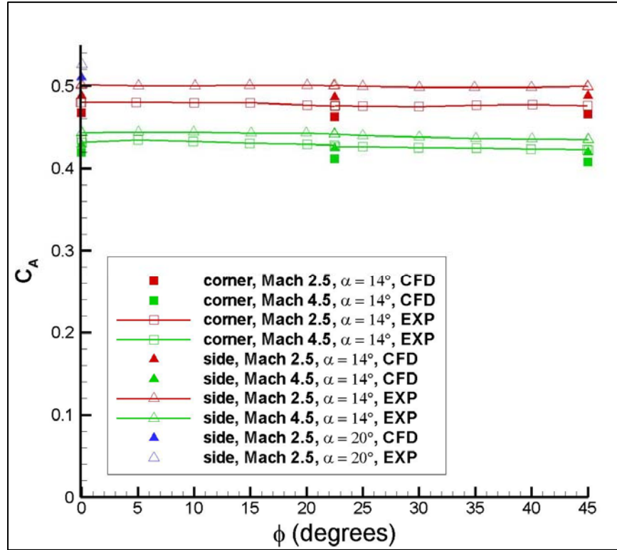
Figure 9. Axial force coefficient as a function of roll orientation.
