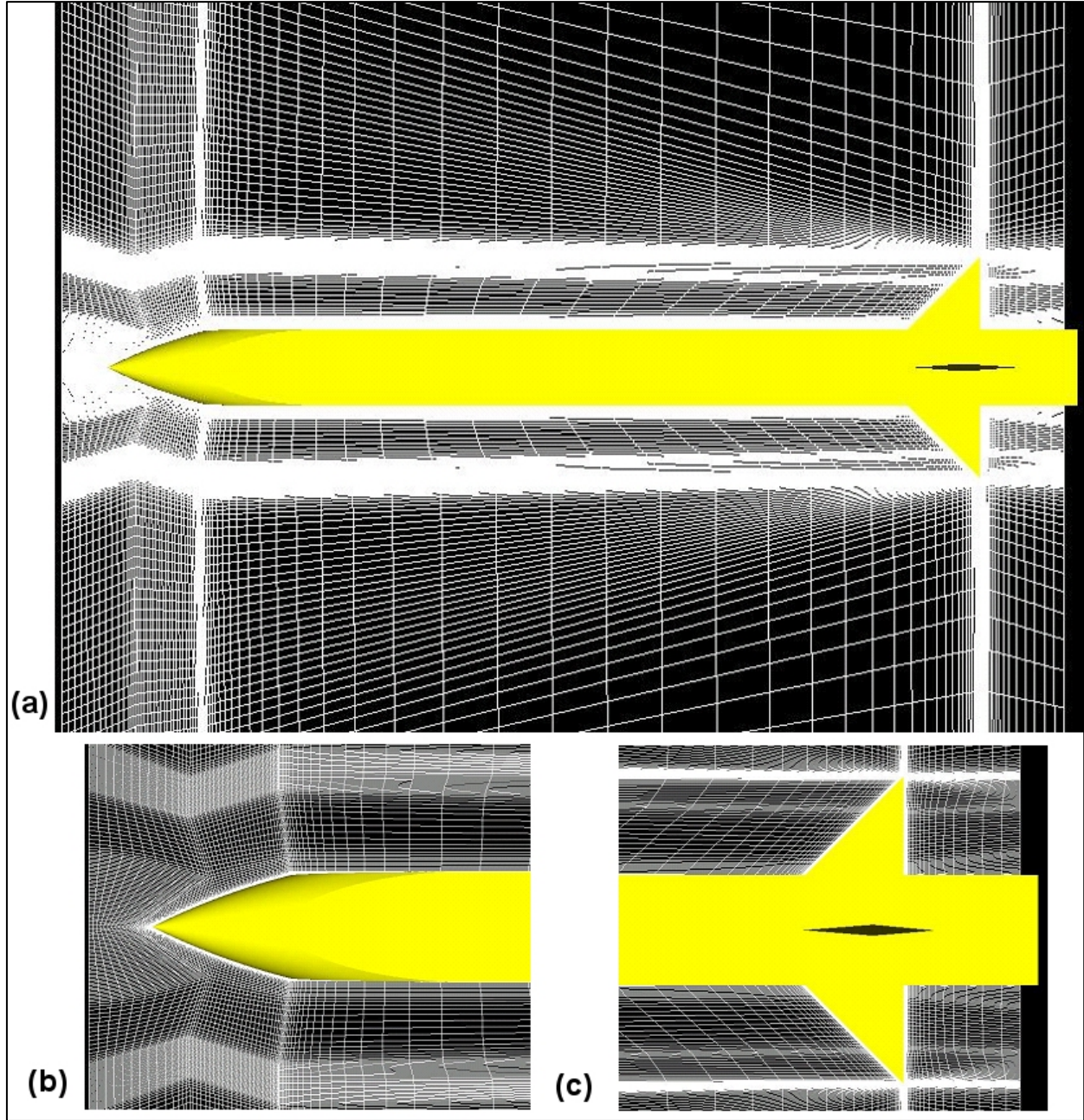
Figure 7. (a) Nine million hexahedral computational grid for side fin geometry with y^+ = 1 spacing. Close-up of (b) nose tip and (c) fins.
