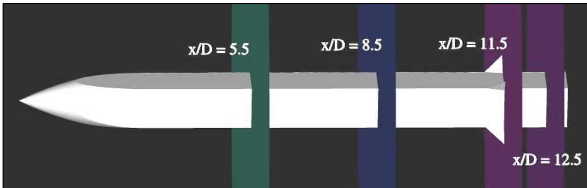
Figure 15. Reference axial body position locations on corner fin configuration.
