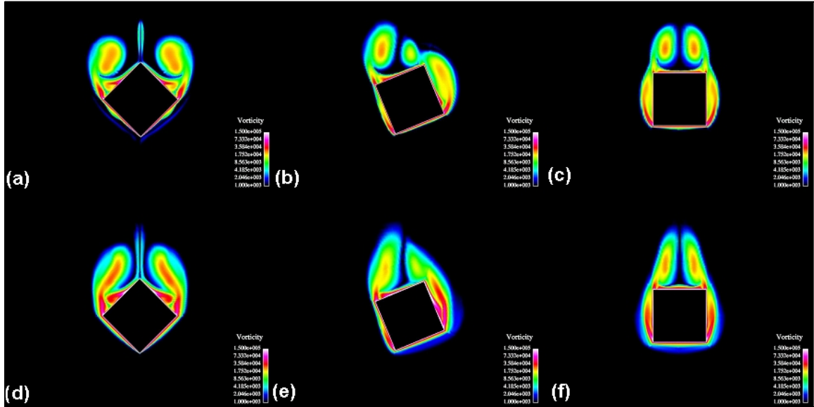
Figure 41. Vorticity contour plots at x/D = 8.5 , \alpha = 14^\circ for corner fin configuration ([a]–[c]) Mach 2.5, \phi = 0^\circ, 22.5^\circ, 45^\circ , respectively, and ([d]–[f]) Mach 4.5, \phi = 0^\circ, 22.5^\circ, 45^\circ , respectively.
