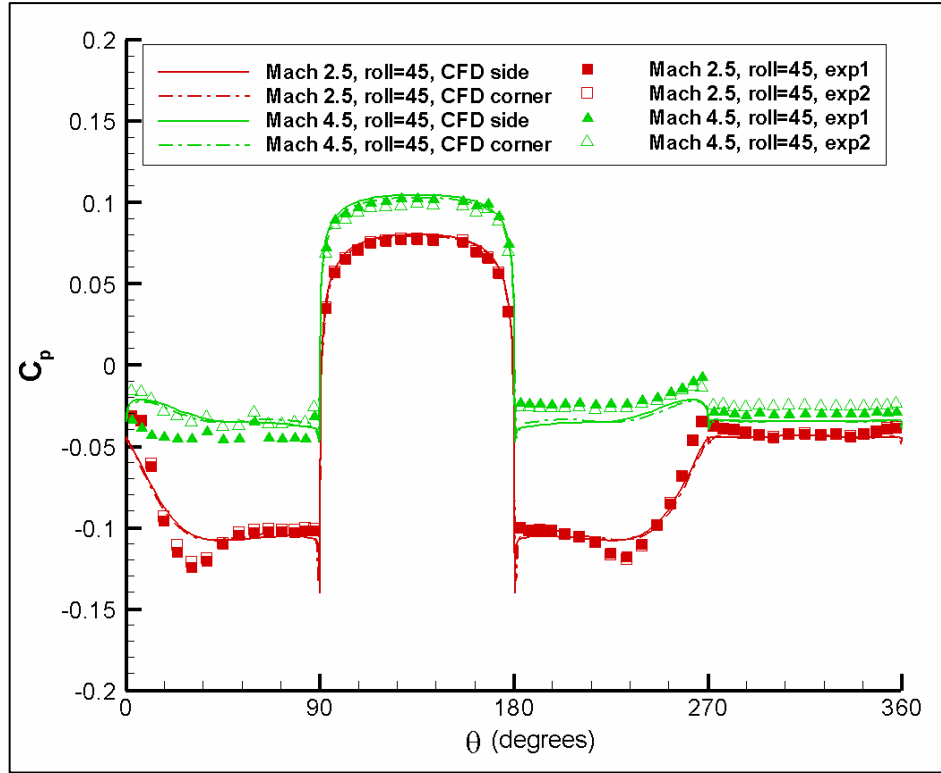
Figure 21. Pressure coefficient distribution at x/D = 8.5 , \phi = 45^\circ , \alpha = 14^\circ .
