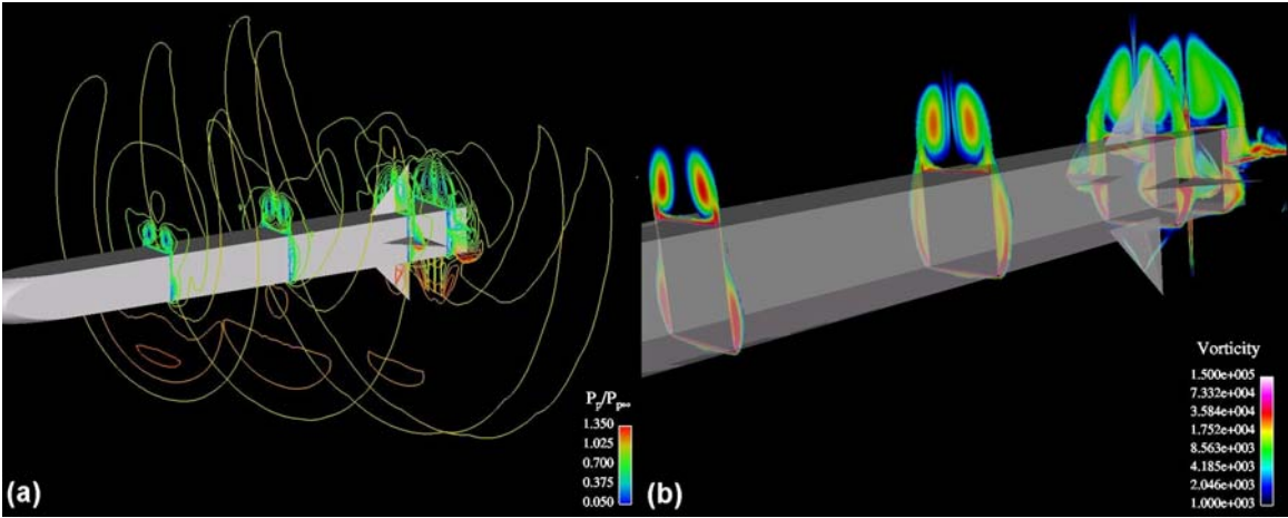
Figure 30. Three-dimensional (a) pitot pressure contours and (b) vorticity contours for side fin configuration, Mach 2.5, \phi = 45^\circ , \alpha = 14^\circ .
