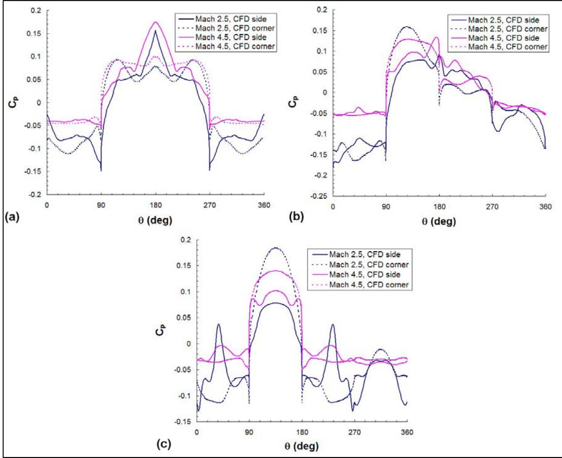
Figure 23. Pressure coefficient distribution at x/D = 12.5 . (a) \phi = 0^\circ , \alpha = 14^\circ , (b) \phi = 22.5^\circ , \alpha = 14^\circ , (c) \phi = 45^\circ , \alpha = 14^\circ .
