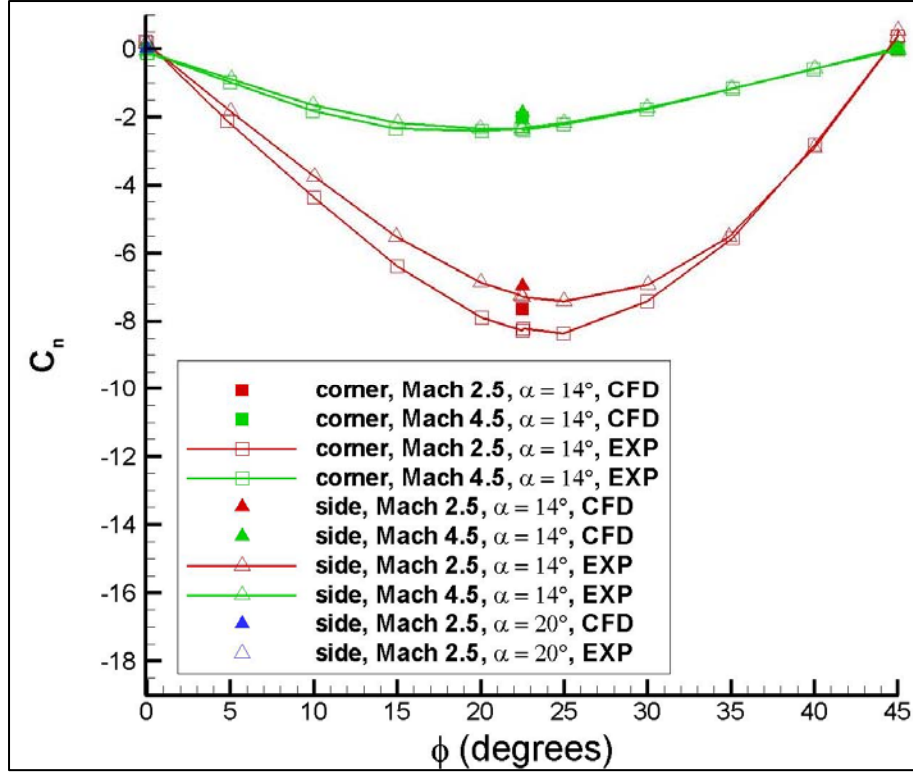
Figure 14. Yawing moment coefficient as a function of roll orientation.
