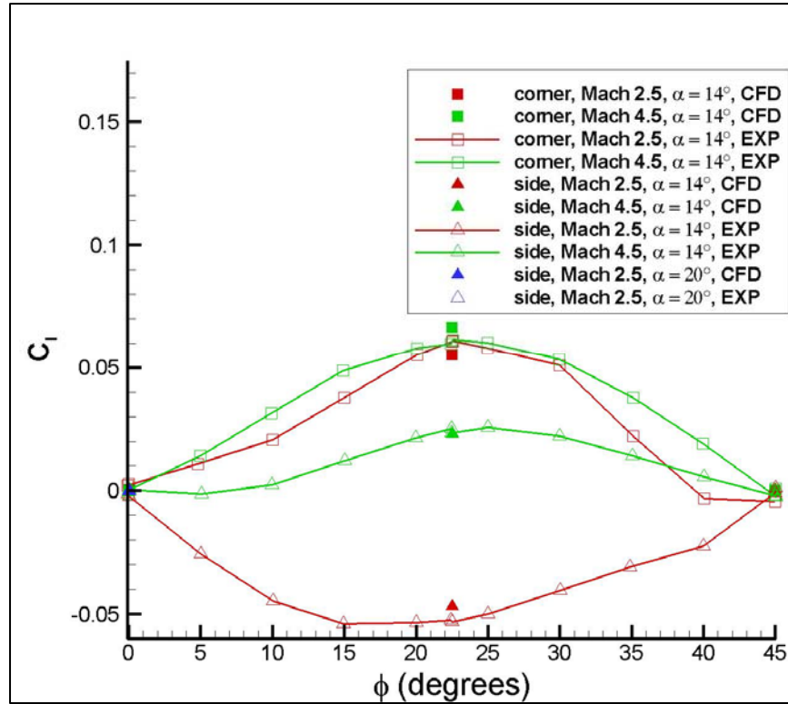
Figure 12. Rolling moment coefficient as a function of roll orientation.
