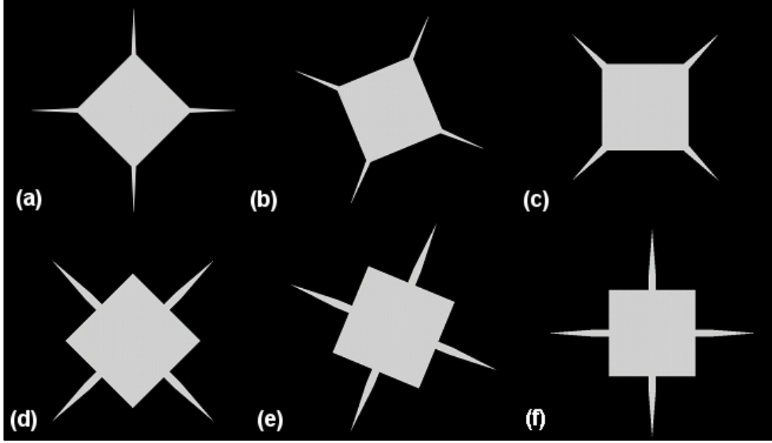
Figure 8. Roll orientation of 0^\circ , 22.5^\circ , and 45^\circ for (a)–(c) corner fin projectile and (d)–(f) side fin projectile looking from projectile base.
