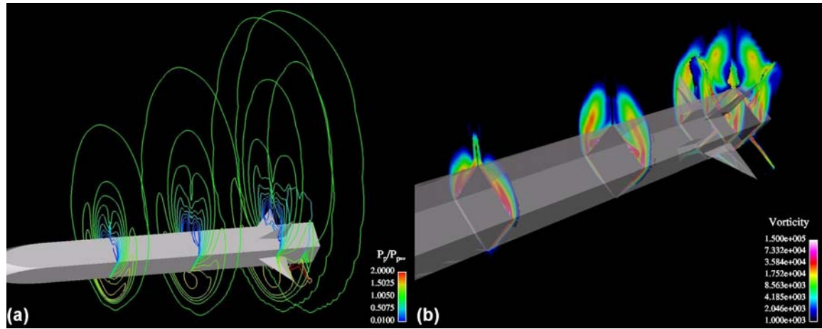
Figure 33. Three-dimensional (a) pitot pressure contours and (b) vorticity contours for side fin configuration, Mach 4.5, \phi = 0^\circ , \alpha = 14^\circ .
