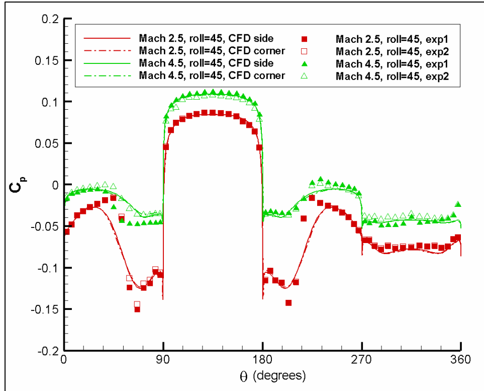
Figure 18. Pressure coefficient distribution at x/D = 5.5 , \phi = 45^\circ , \alpha = 14^\circ .
