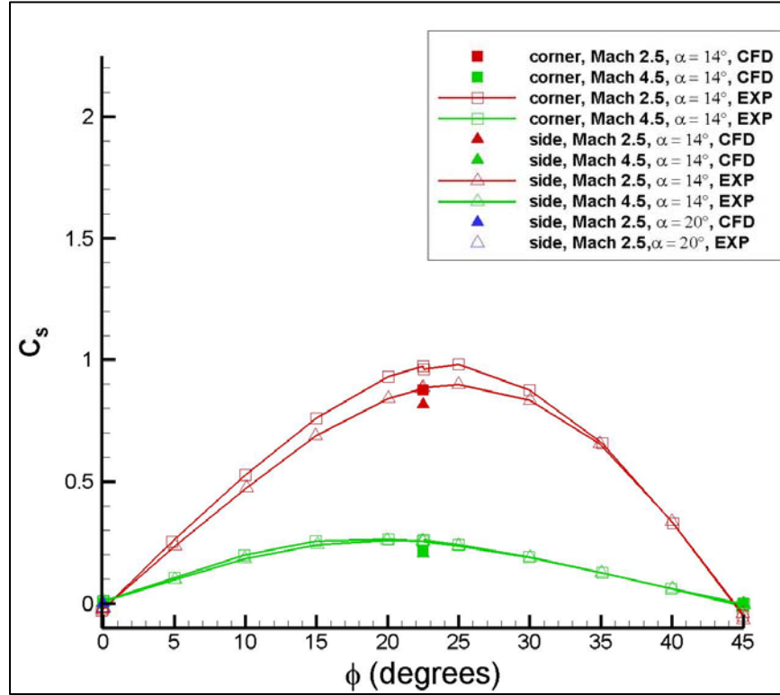
Figure 11. Side force coefficient as a function of roll orientation.
