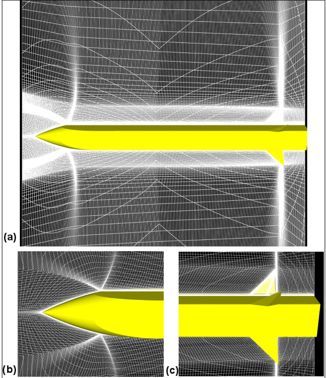
Figure 6. (a) Computational grid for corner fin geometry with y^+ = 1 spacing. Close-up of (b) nose tip and (c) fins.
