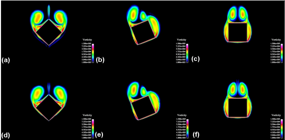
Figure 39. Vorticity contour plots at x/D = 8.5 , Mach 2.5, \alpha = 14^\circ for ([a]–[c]) corner fin configuration \phi = 0^\circ, 22.5^\circ, 45^\circ , respectively, and ([d]–[f]) side fin configuration, \phi = 0^\circ, 22.5^\circ, 45^\circ , respectively.
