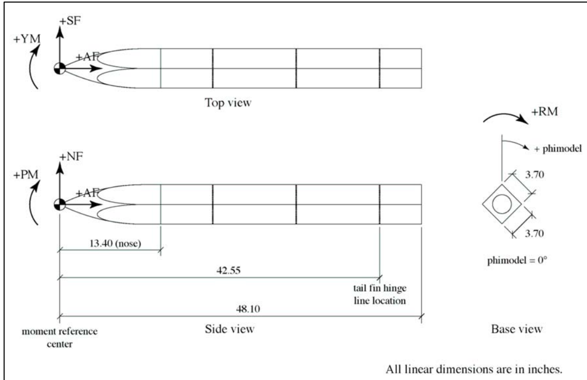
Figure 1. Reference dimensions and orientation for the square section missile, no fins.
