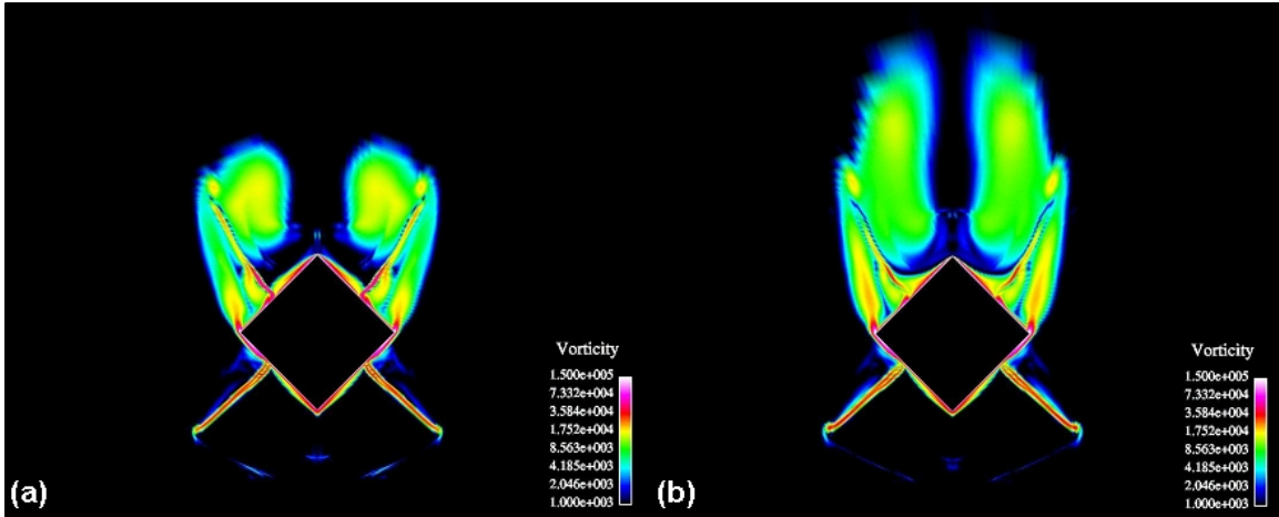
Figure 48. Vorticity contours for side fin configuration at Mach 2.5, \alpha = 0^\circ , x/D = 12.5 , (a) \alpha = 14^\circ and (b) \alpha = 20^\circ .
