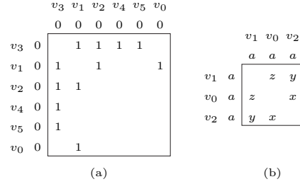
Figure 3: Canonical adjacency matrices
