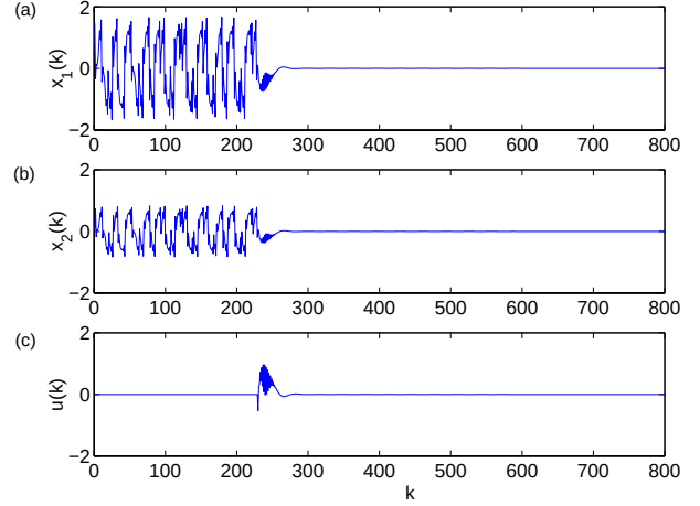
Fig. 1. Time series (with initial condition (1.4725, 0.0557)) of (a) x_1 (b) x_2 and (c) control input u . The control is applied when the trajectory of the open-loop system enters the neighborhood \{x = (x_1, x_2) \in \mathbb{R}^2 : \|x\| < 0.1\} of the origin.
