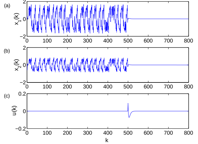
Fig. 2. Time series (with initial condition (0.3,-0.6)) of (a) x_1 (b) x_2 and (c) control input u . The control is applied when the trajectory of the open-loop system enters the neighborhood \{x = (x_1, x_2) \in \mathbb{R}^2 : \|x\| < 0.15\} of the origin.
