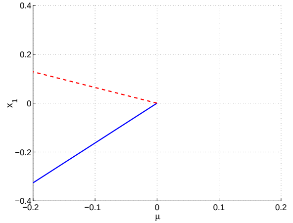
Fig. 4. Bifurcation diagram for Example 3 without control. The solid line represents a path of stable fixed points whereas the dashed line represents a path of unstable fixed points.
