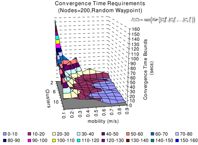
Figure 6 Convergence Time Bounds for cost function (1)
