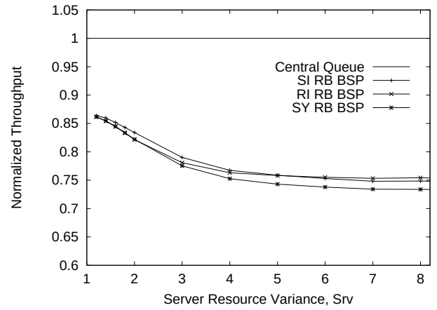
(e) Server Resource Correlation: Src=0.50
