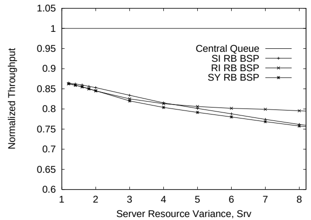
(f) Server Resource Correlation: Src=0.70
