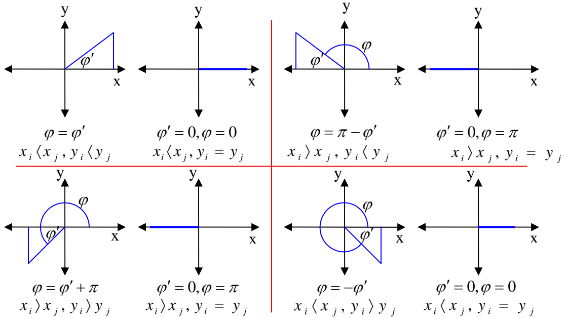
Figure 16. \phi Defined For All Combinations of x-y Coordinates of Two Nodes [Adapted from 6].
