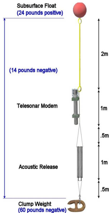
Figure 1. Seaweb Node [From 1].
