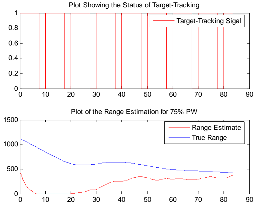
Figure 23. Plot of the Range Estimation for 25% Target-Tracking Error
