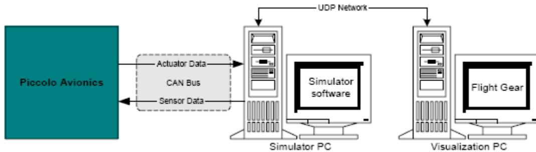
Figure 4. HIL Simulation. (From: [Ref. 6])
