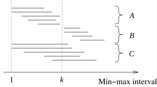
Figure 7: Min-max intervals of a set of sequences.
