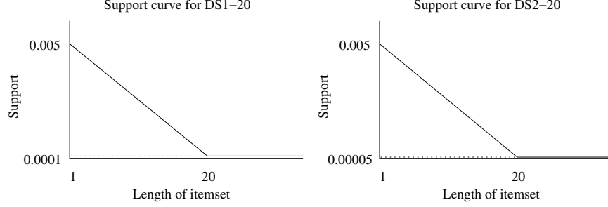
Figure 8: Support curve for DS1-20 and DS2-20.
