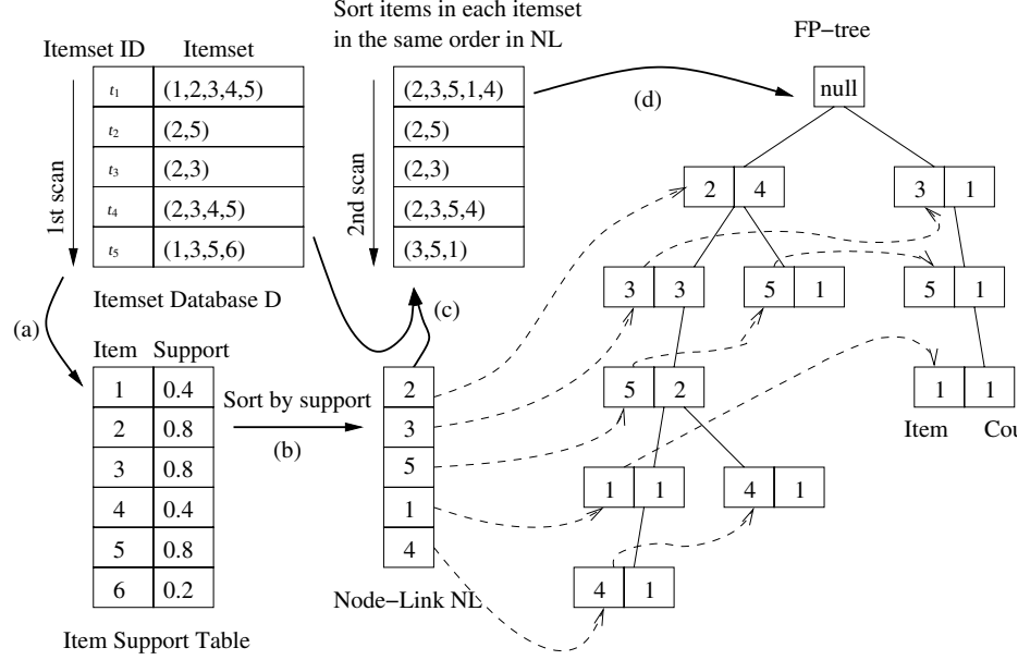
Figure 3: Flow of FP-tree generation.
