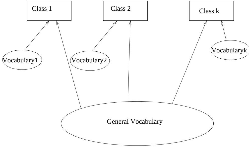
Figure 4: Document Model
