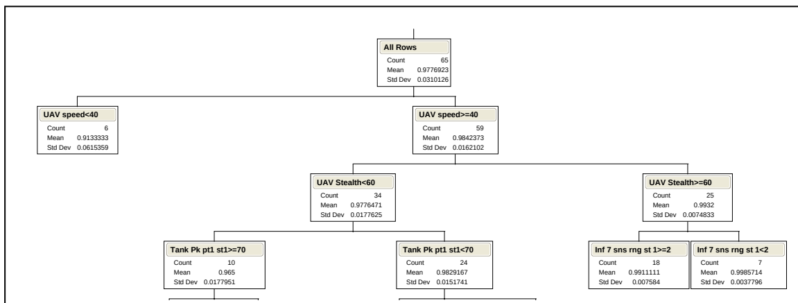
Figure 14. Regression Tree for the Base Case. Shows Speed and Stealth as the first two break points.
