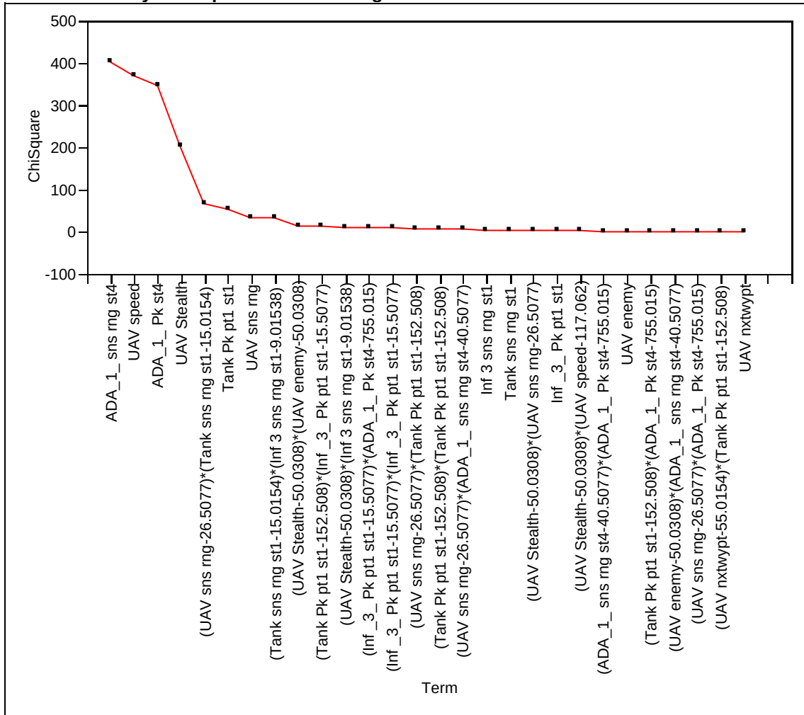
3X Threat Desity Chi Square Value Per Significant Term
