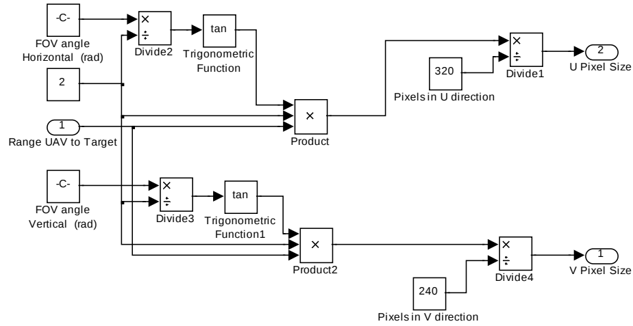
Figure 32. Compute Pixel Size Block.
