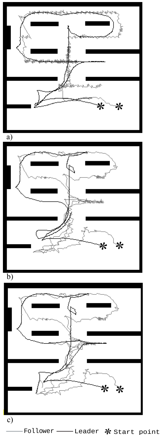
Figure 2: The traces of leader and follower controlled by the three controllers in the same maze: a) line-of-sight exploration, 720 control cycles; b) line-of-sight exploration with collaborative search, 531 control cycles; c) line-of-sight exploration with both collaborative search and role-change, 492 control cycles and 3 role-changes.
