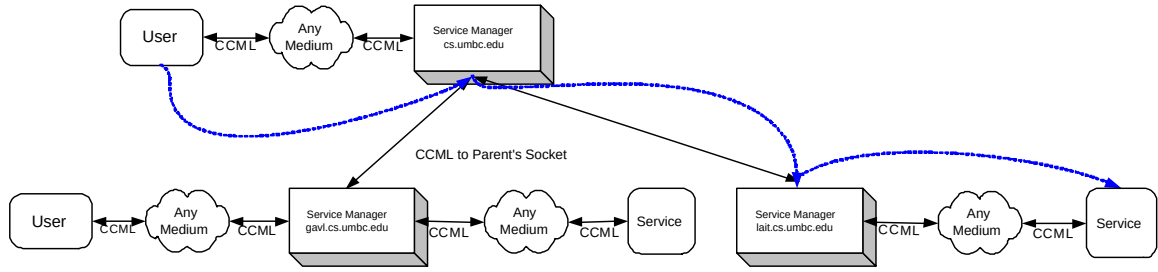
Fig. 5. Multiple Service Manager Registrations
