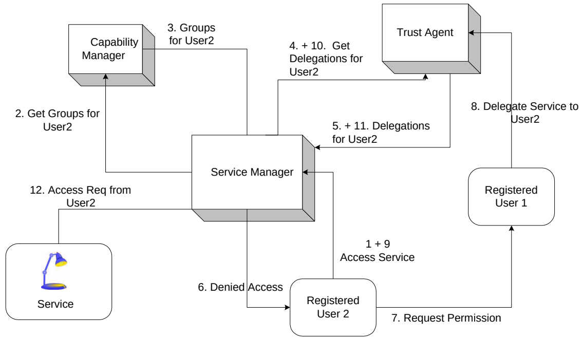
Fig. 3. Trust Agent Functionality
