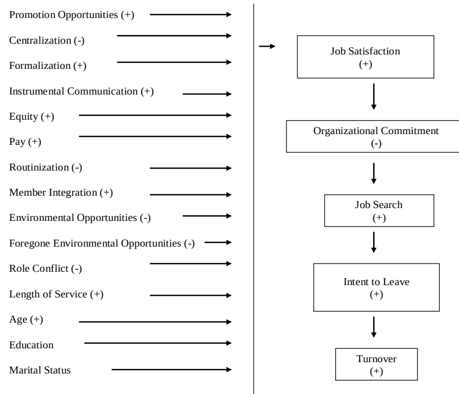
Appendix A, Figure A7: Unified Model of Turnover
