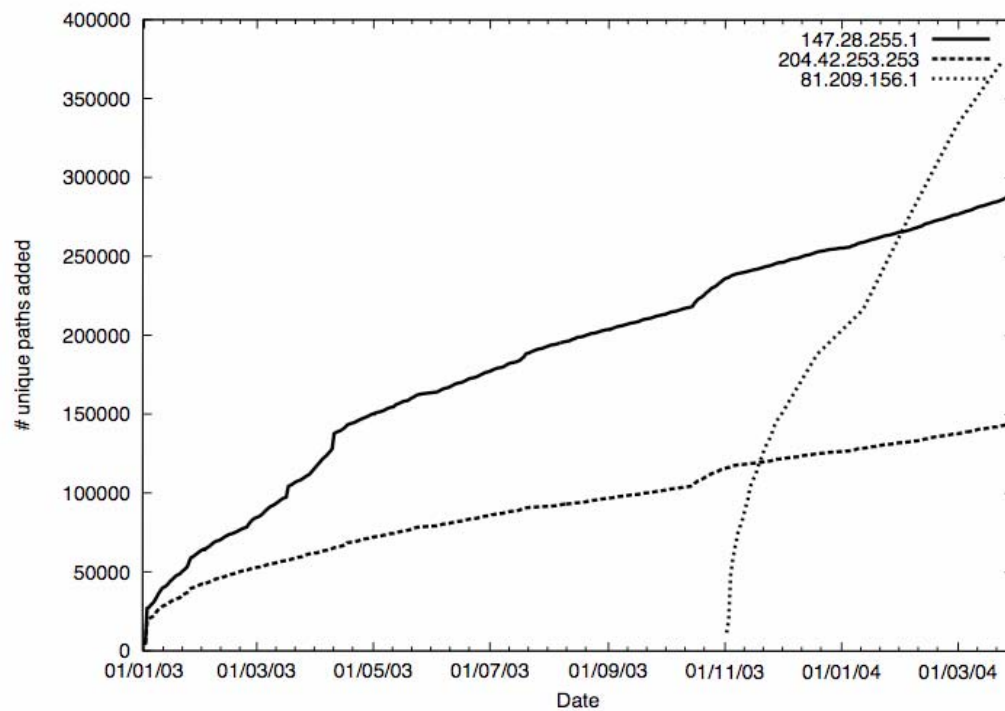
Figure 60. Rate of Discovery: the number of new unique paths discovered aggregated by AS. This graph shows that for all listeners, there are relatively few new unique paths added on a daily or weekly basis, another good signaling indicator.
