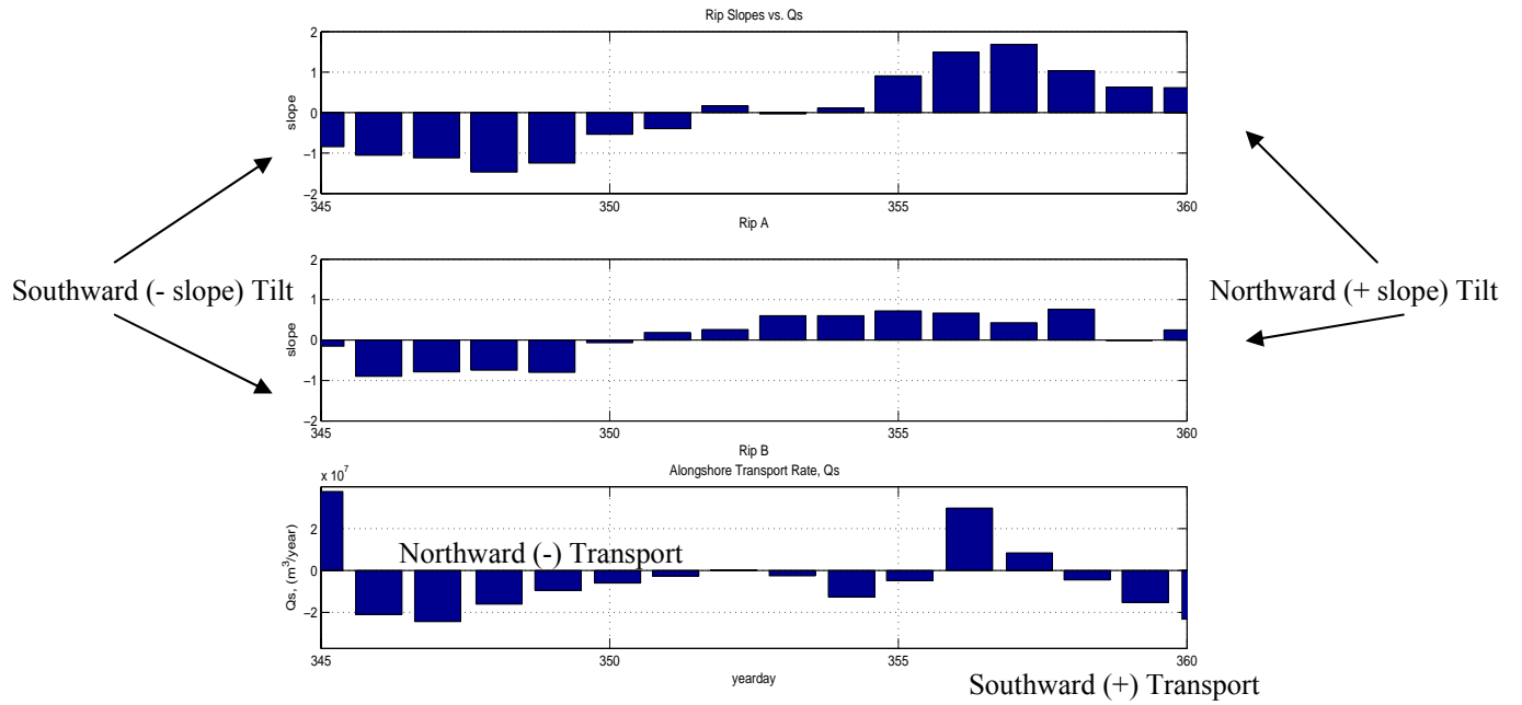
Figure 17. Rip channels A and B tilts from Figure 16 slopes vs. Q_s . The rip channels tilt in the direction opposite to sediment transport. The base of the rip channels migrate faster than the offshore portion of the rip channel causing a tilting in the opposite direction.
