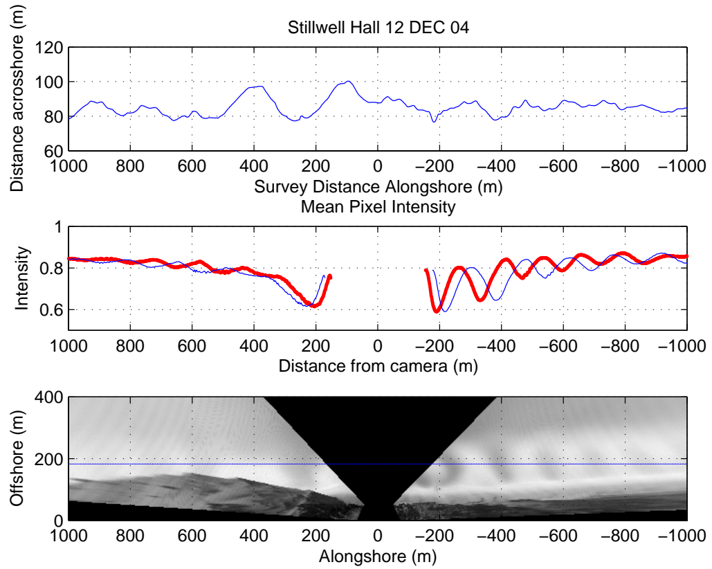
Figure 9 Data used for correlation between ATV survey data and mean pixel intensity line is 2m contour data from ATV survey. Middle panel is mean pixel intensity line at 180m before camera correction (blue line) and after correction (red line). Bottom panel is a daytimex image for corresponding day.
