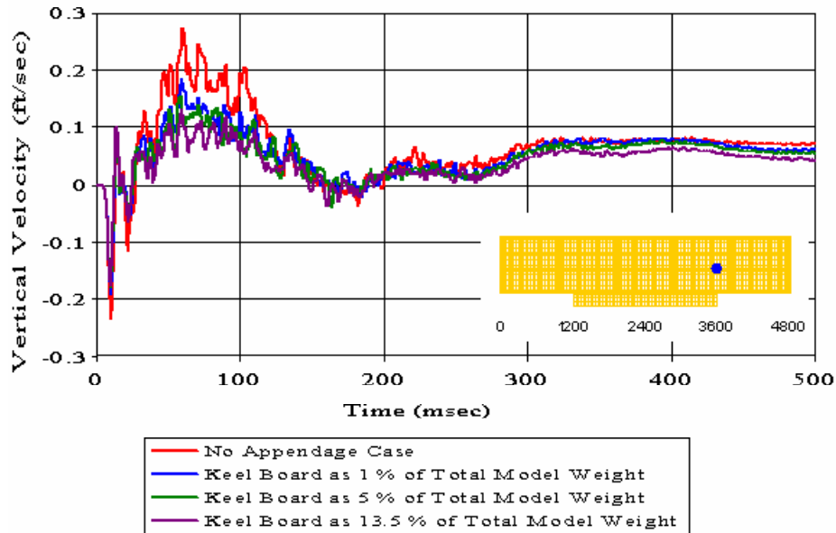
Figure 164. Uncoupled Case with Varying Weight Percentage: First Deck Node 8364
