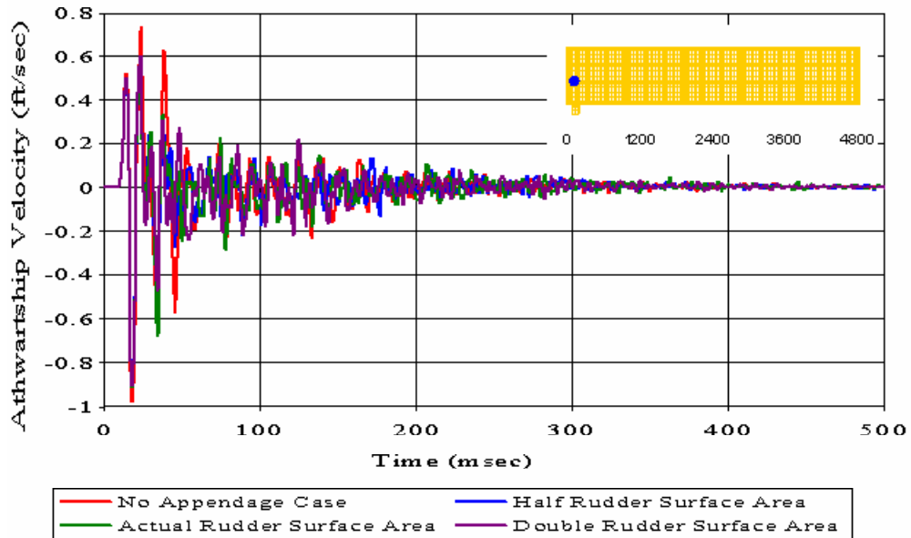
Figure 390. Coupled Case with Varying Rudder Surface Area: First Deck Node 214
