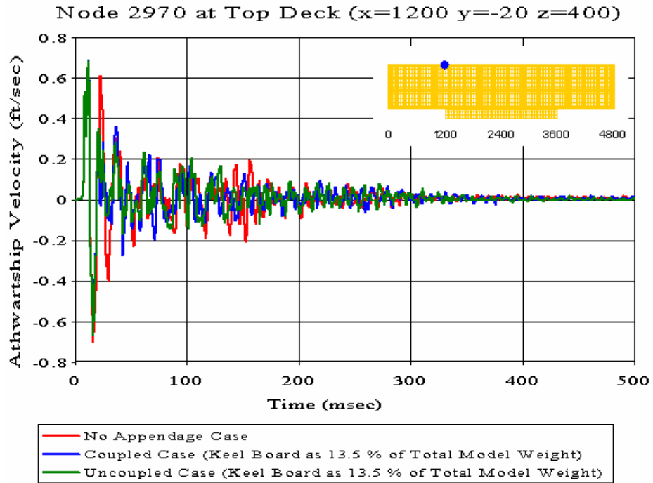
Figure 274. Top Deck Node 2970: (RM = -0.0217, RP = 0.1939, RC = 0.1729)
