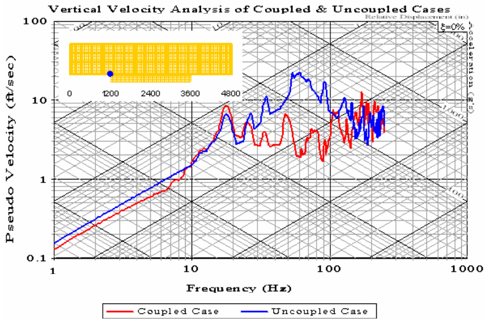
Figure 65. Shock Spectra Plot: Keel Node 2454
