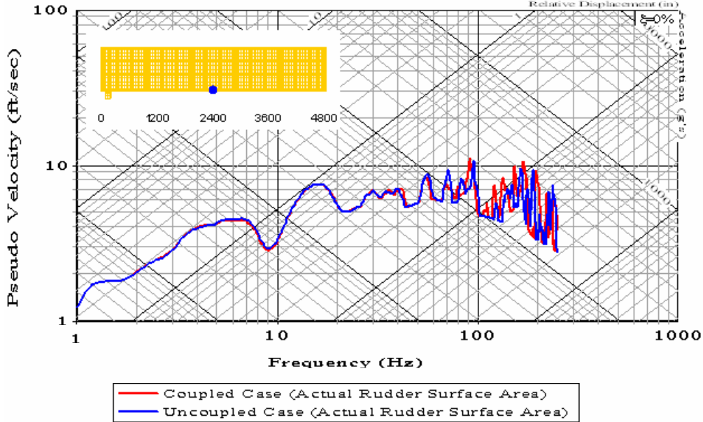
Figure 478. Shock Spectra Plot: Keel Node 5308
