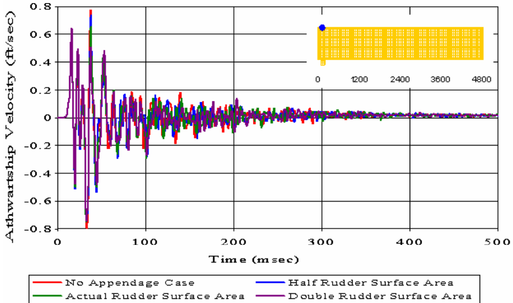
Figure 416. Uncoupled Case with Varying Rudder Surface Area: Top Deck Node 434
