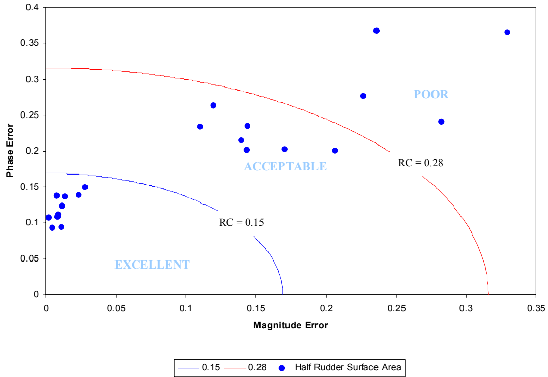
Figure 496. Russell's Error Factor Comparison for Meko-Like Box Model with Rudders Having Half Rudder Surface Area (Athwartship Velocity)
