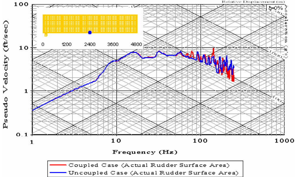
Figure 479. Shock Spectra Plot: Keel Node 5315
