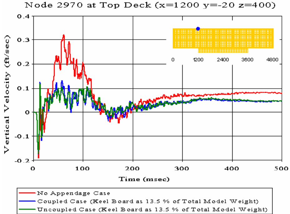
Figure 110. Top Deck Node 2970: (RM = -0.0003, RP = 0.0783, RC = 0.0694)
