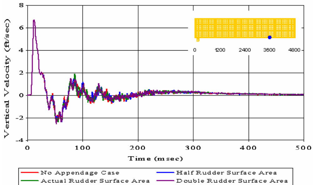
Figure 268. Uncoupled Case with Varying Rudder Surface Area: Keel Node 8170
