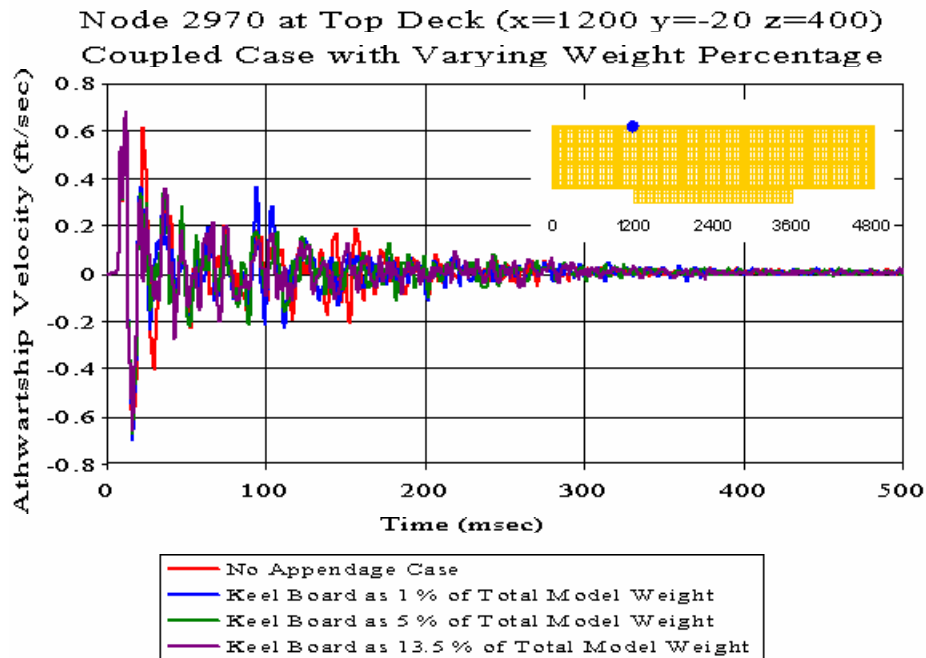
Figure 295. Coupled Case with Varying Weight Percentage: Top Deck Node 2970
