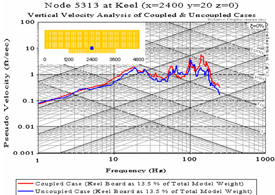
Figure 54. Shock Spectra Plot: Keel Node 5313
