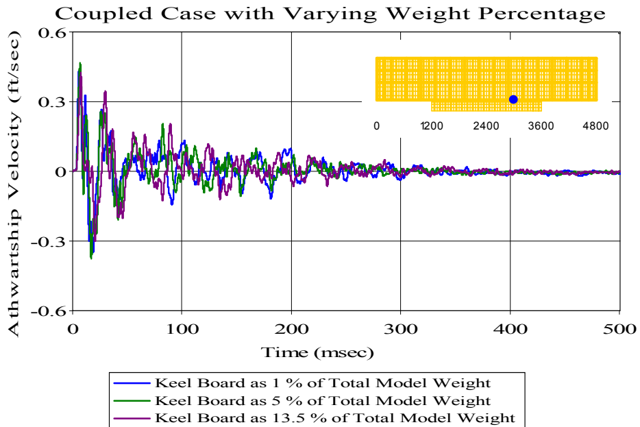
Figure 305. Coupled Case with Varying Weight Percentage: Keel Node 6741
