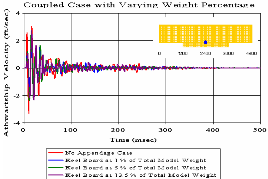
Figure 304. Coupled Case with Varying Weight Percentage: Keel Node 5320
