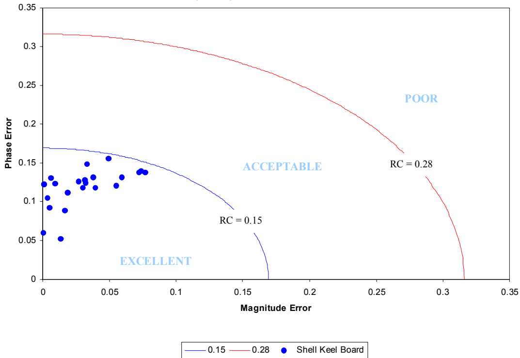
Figure 59. Russell's Error Factor Comparison for Meko-Like Box Model with Shell Keel Board (Athwartship Velocity)
