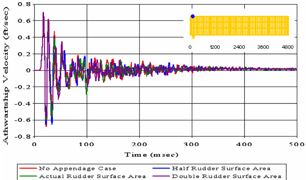
Figure 417. Uncoupled Case with Varying Rudder Surface Area: Top Deck Node 441
