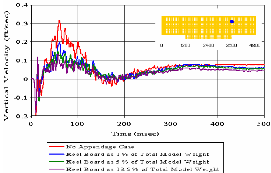
Figure 165. Uncoupled Case with Varying Weight Percentage: Second Deck Node 8536
