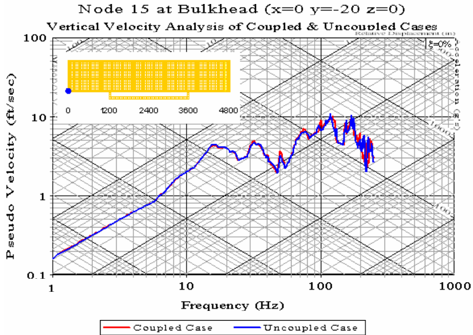
Figure 461. Shock Spectra Plot: Bulkhead Node 15
