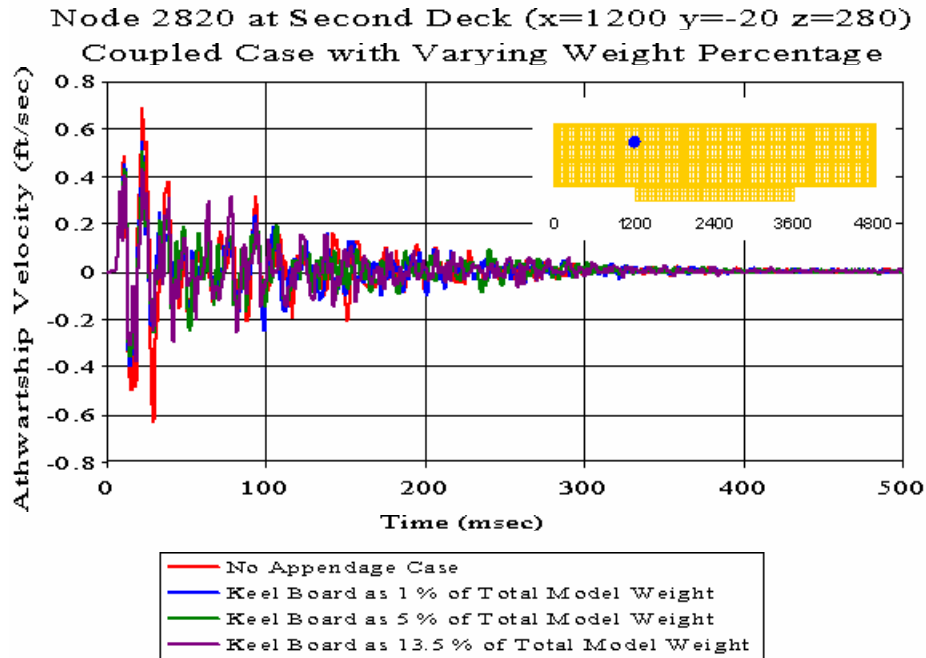
Figure 294. Coupled Case with Varying Weight Percentage: Second Deck Node 2820
