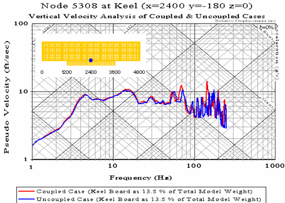
Figure 55. Shock Spectra Plot: Keel Node 5308
