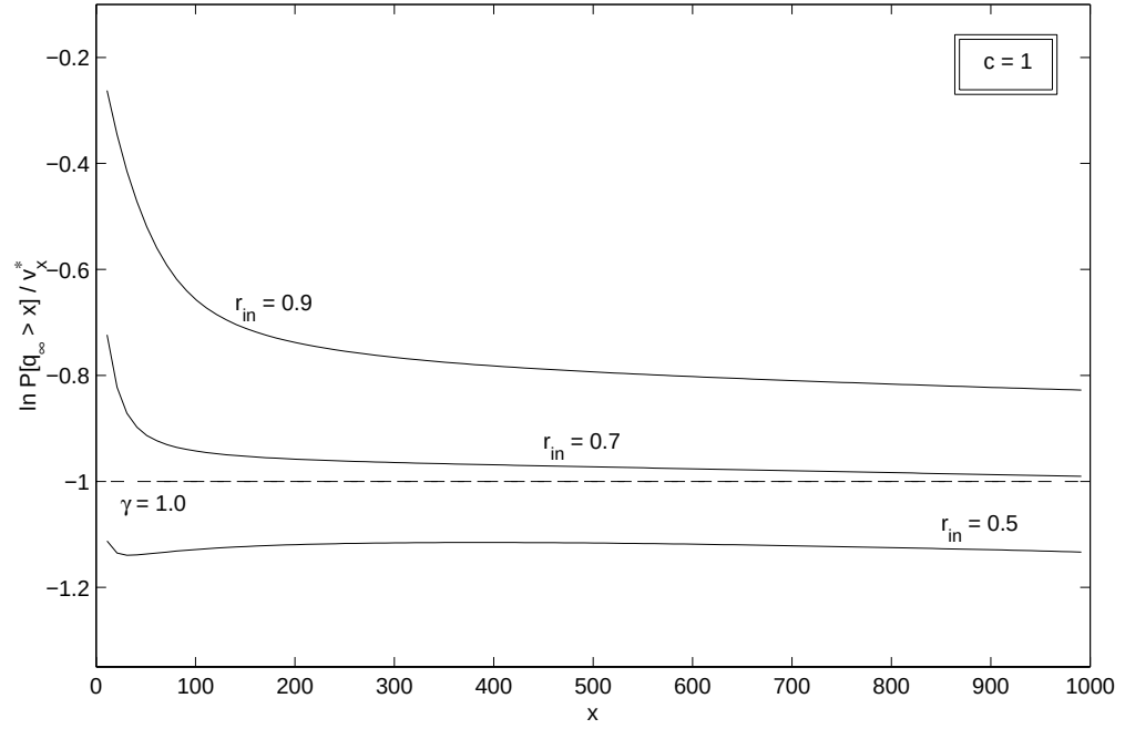
Figure 17: Tail probability vs. buffer size: Pareto ( \alpha = 2.5 )
