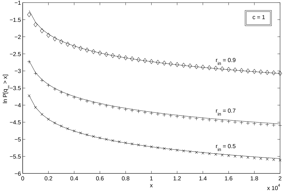
Figure 20: Pareto ( \alpha = 1.5 )
