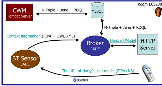
Figure 3: In our prototype system, the broker attempts to infer the location context of devices and users. An user model is dynamically acquired from an URL specified in the received user policy.
