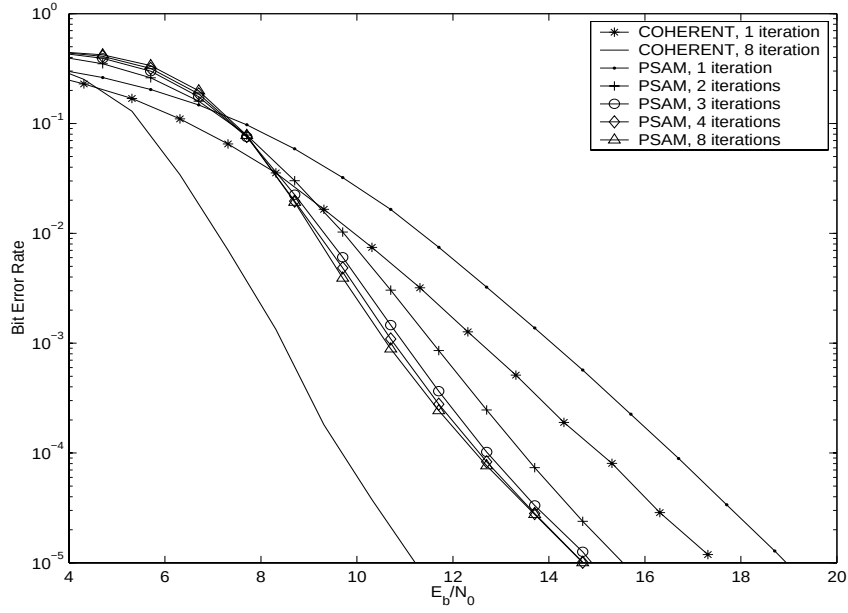
Figure 2.6: Performance of the PSAM receiver with iterative demodulation and decoding ( f_D T = 0.01 )
