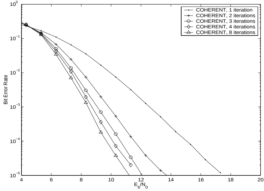
Figure 2.5: Performance of the coherent CPM receiver with iterative demodulation and decoding ( f_D T = 0.01 )
