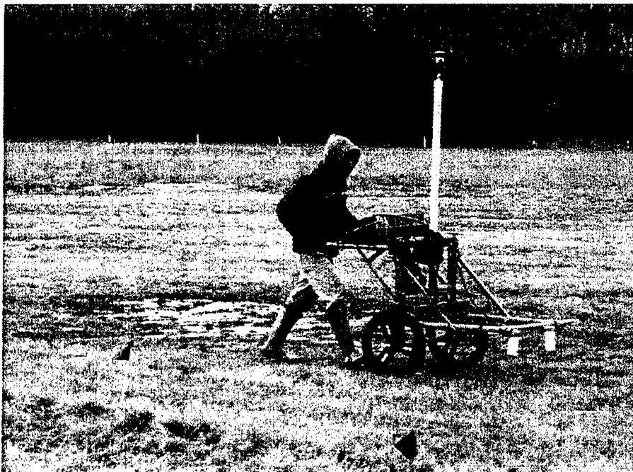
Figure 1. Shaw UXO Mapper (dual sensor G858 magnetometer).
