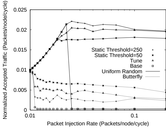
Figure 5. Static Threshold vs. Tuning.
