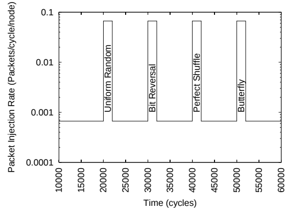
Figure 6. Offered bursty load
