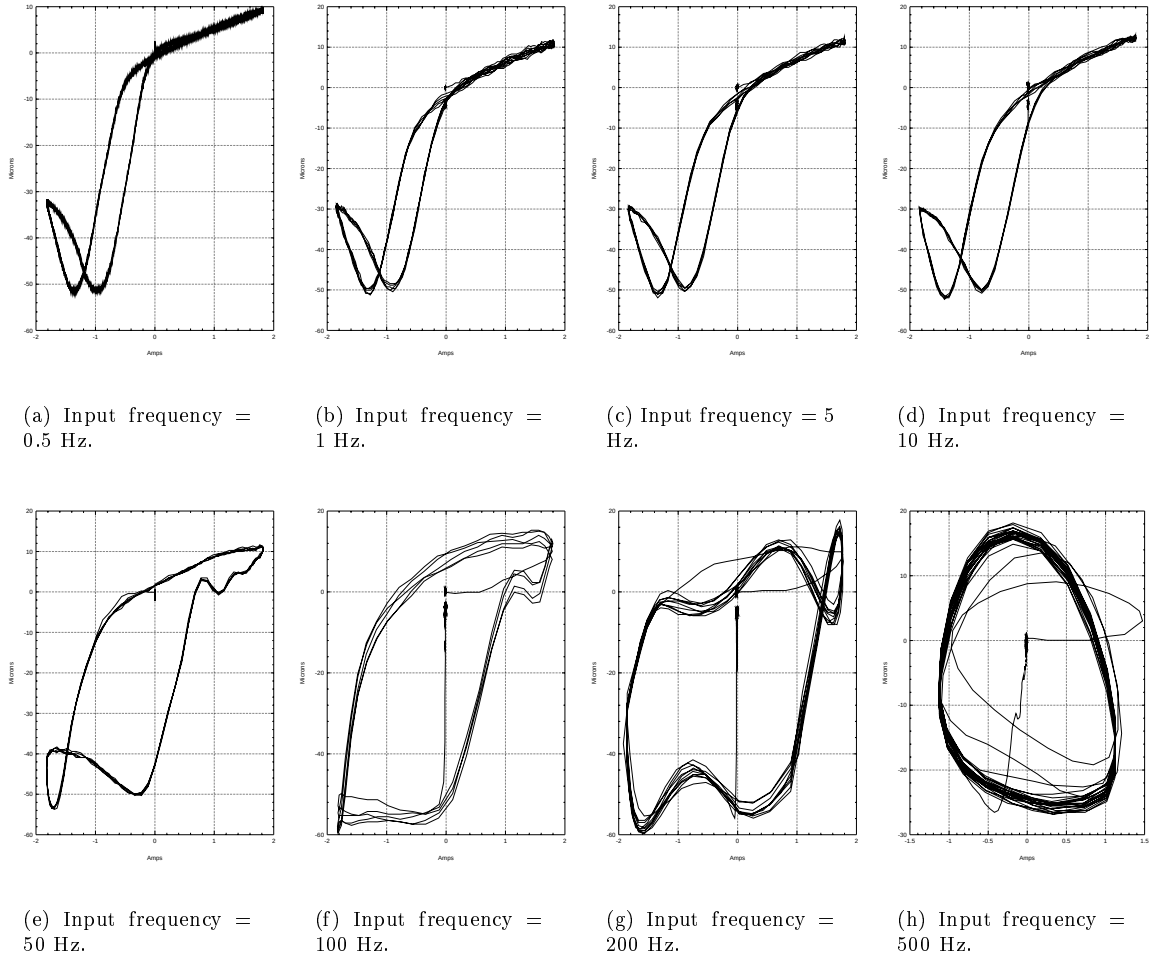
Figure 9: ETREMA MP 50/6 Actuator characteristic at different driving frequencies.
