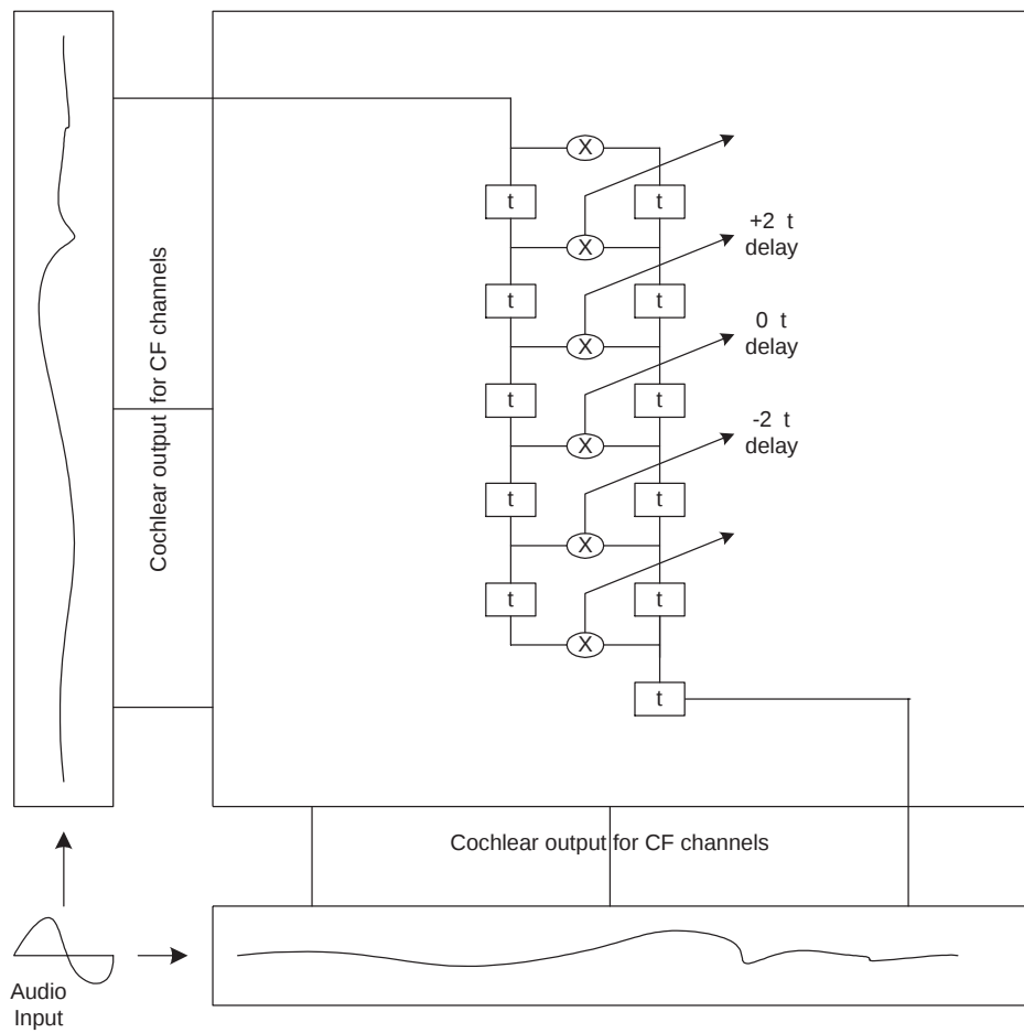
Figure 3.5: The Jeffress network.
