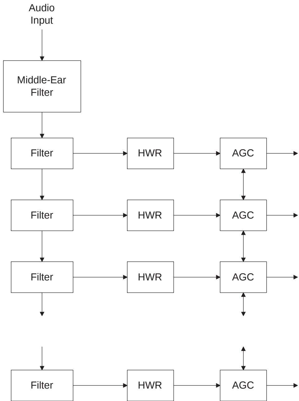
Figure 3.1: Lyon's cochlear model.
