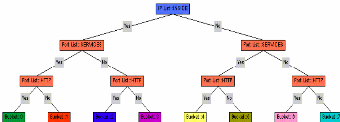
Figure 17. [After KAHWAI-04] A decision tree for the HTTP PID instance. This is the tree used in the Apache 2 attack shown in Figure 14.
