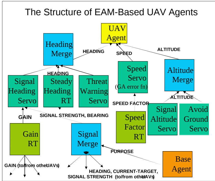
Figure 3. The Multi-Level EAM Control Structure in a UAV Agent System
